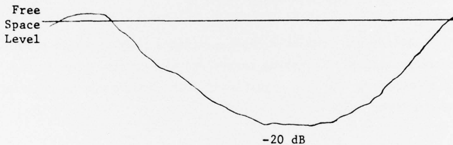
Figure 5. Typical AGC recording of obstruction type fading
