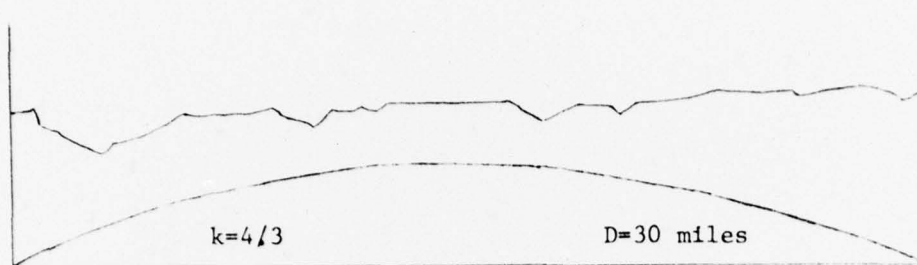
Figure 8. Path profile
