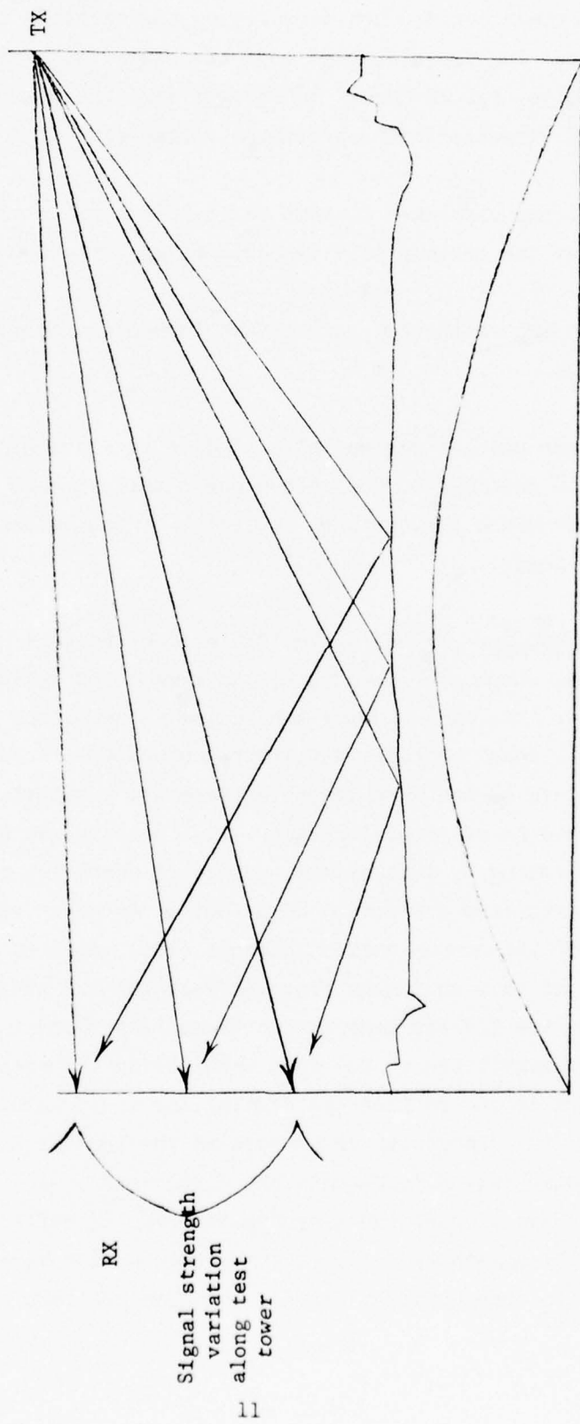
Figure 6. Interference pattern
