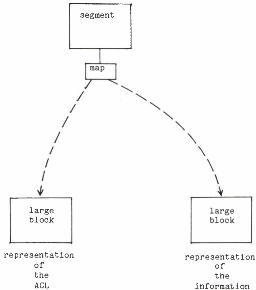
Figure 4-4 Actual Representation Objects for Segments
