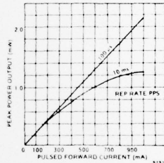
Figure 6 Peak Power Output vs. Pulsed Forward Current
