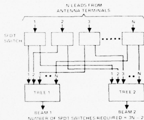
(b) SWITCHING MATRIX USED TO SELECT TWO SIMULTANEOUS BEAM POSITIONS. THE TWO SWITCHING TREES ARE IDENTICAL TO THAT SHOWN IN FIG. 1
