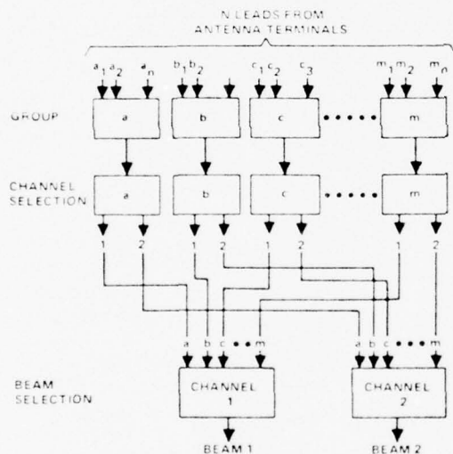
(c) ALTERNATE SWITCHING MATRIX FOR THE SELECTION OF TWO SIMULTANEOUS BEAM POSITIONS. THE TWO BEAMS CANNOT BE SELECTED FROM THE SAME GROUP
