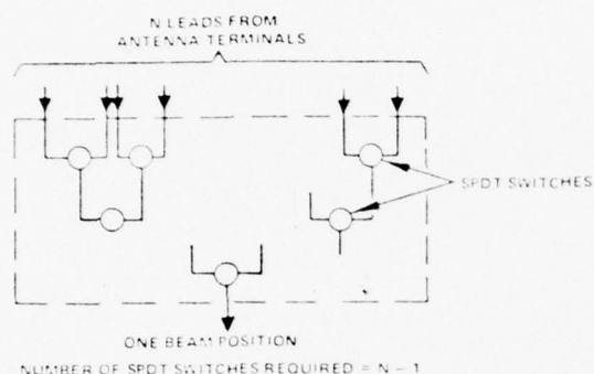
(a) SWITCHING MATRIX USED TO SELECT ONE BEAM POSITION FROM A TOTAL OF N AVAILABLE BEAM POSITIONS
