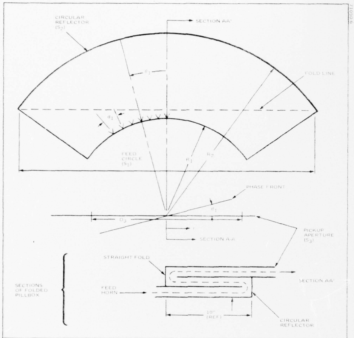
Figure IV.2. Circular Pillbox
