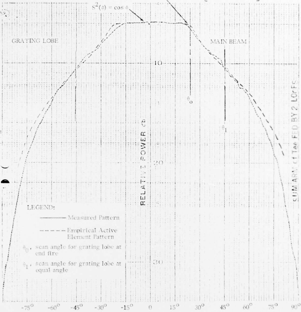
FIGURE C.1 – ACTIVE ELEMENT PATTERN FOR APERTURE FIELD CALCULATION.
