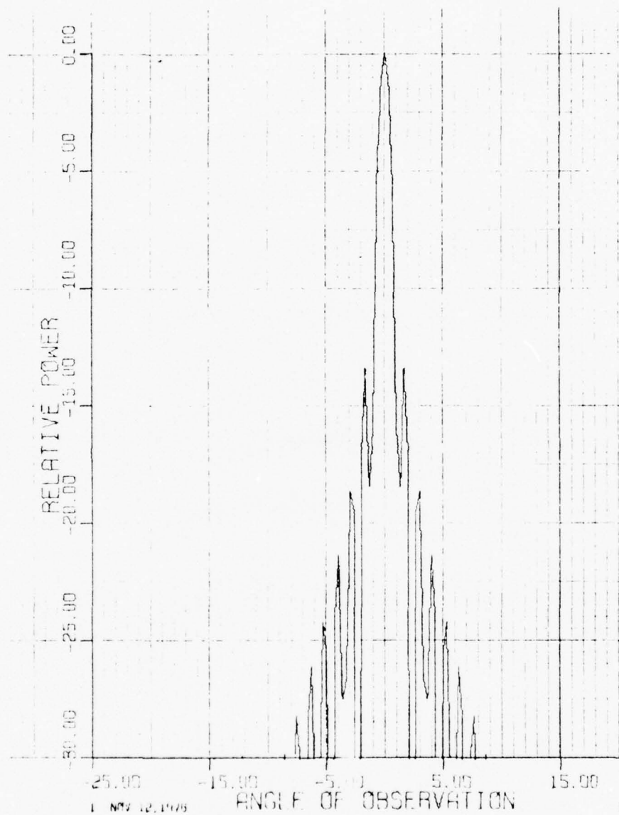
FIGURE V.5 - FAR FIELD PATTERN OF ARRAY WITH SPHERICAL LENS BEAMFORMER 3.0 dB BEAM CROSSOVER 1.55 BEAM COUPLING LOSS
