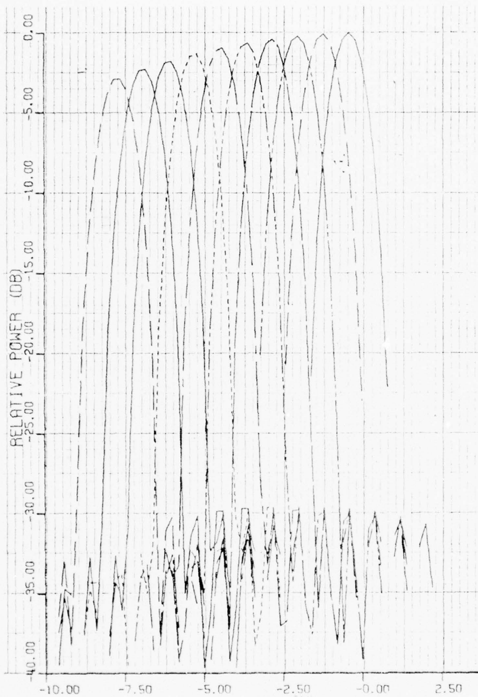
FIGURE IV.16 - FAR FIELD PATTERNS FOR BLOCK FEEDING OF TWO HORNS AND RESISTIVE TAPERING.
