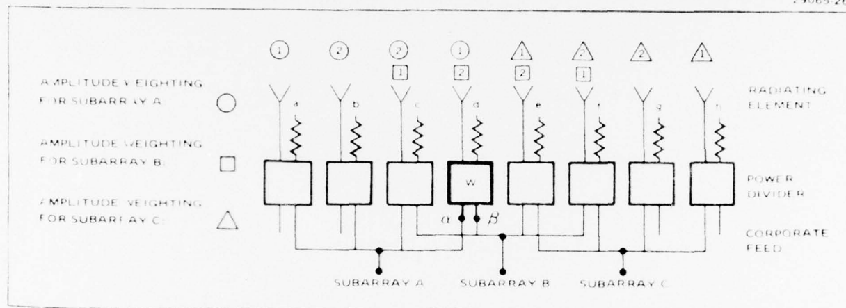
FIGURE III.2 - COUPLING NETWORK IN THE OVERLAPPING SUBARRAY APPROACH.
