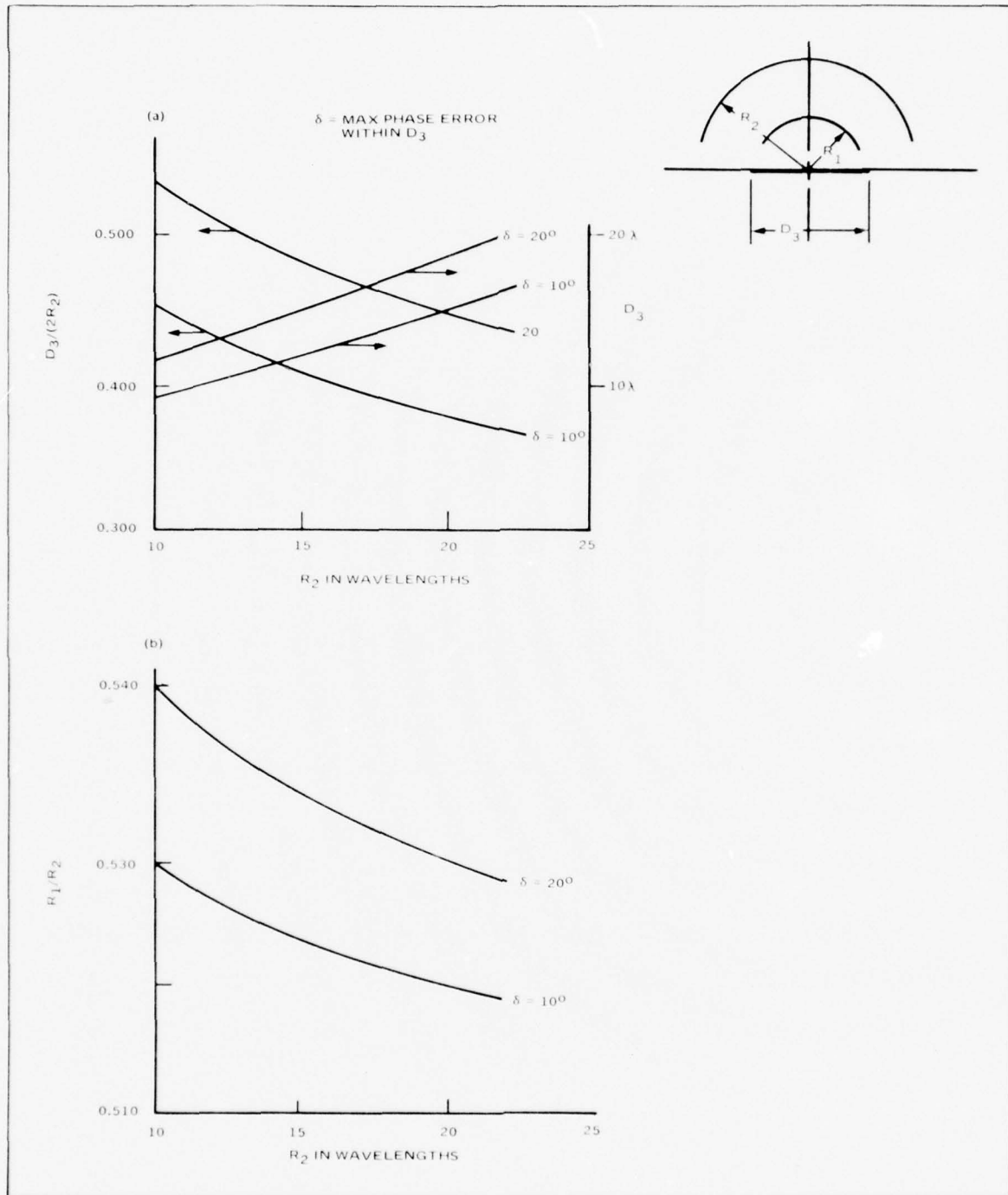
Figure IV.4. Selection of Design Parameters to Meet Specified Allowable Phase Error (Before Compensation)
