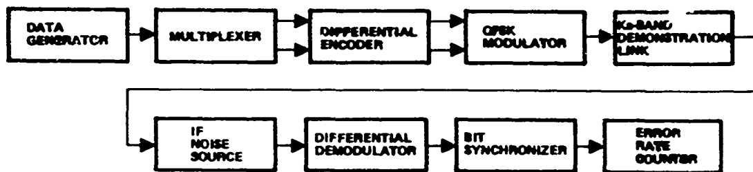
Figure 28. Differentially Coherent QPSK Demonstration Link Test Configuration BER Tests
