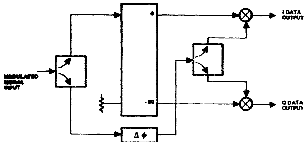
Figure 43. Differential Demodulator
