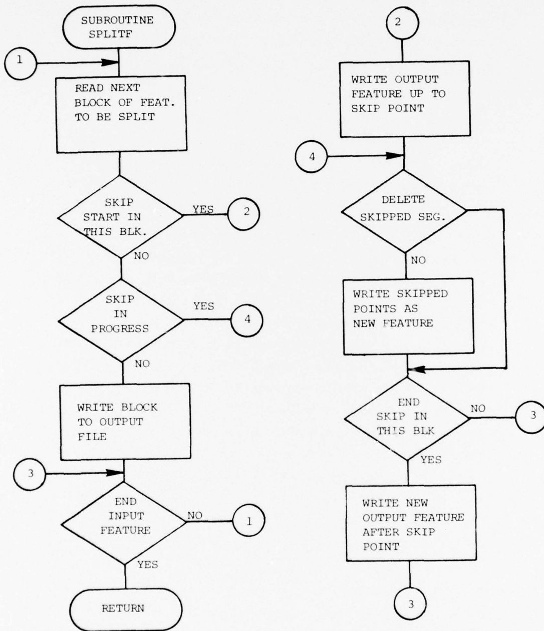
SPLIT FUNCTIONAL FLOW
