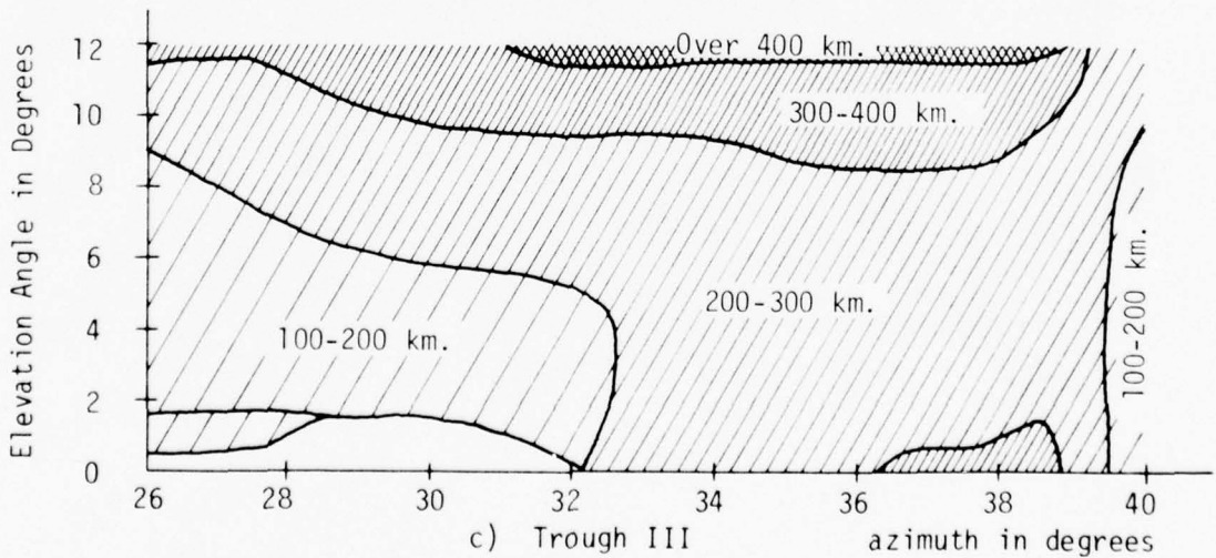
FIGURE 16. RANGE ERRORS USING 3.0 MHz STANDARD FOR 5 MHz TRANSMISSION FREQ.
