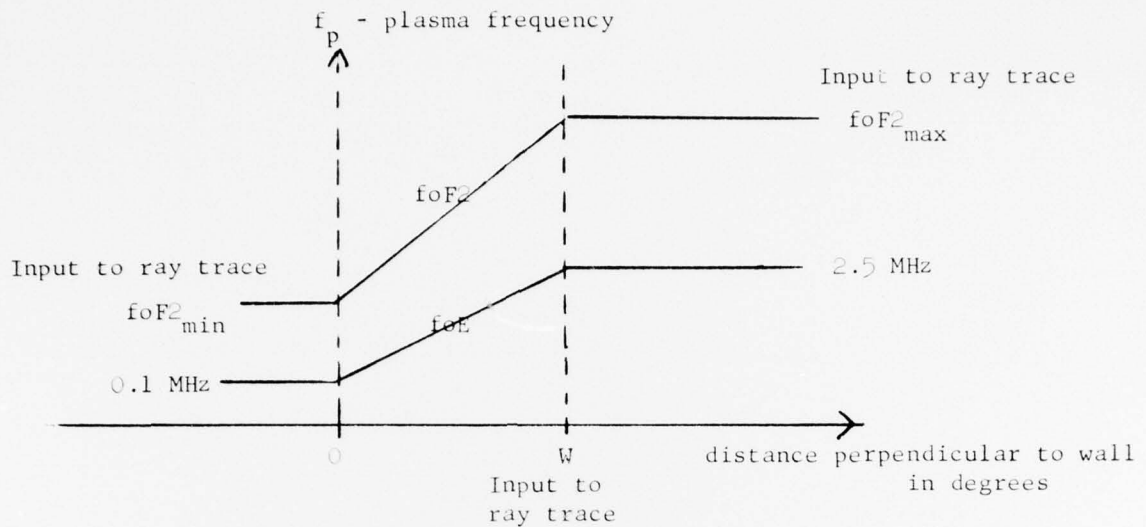
Figure 2. Variation of foE and foF2 across the Trough Wall
