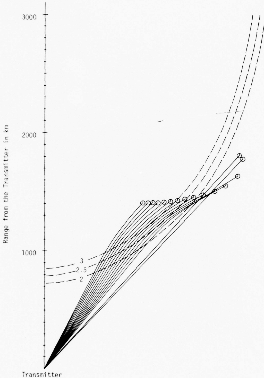
FIGURE 19. RAY PATHS PLOTTED AS A FUNCTION OF RANGE AND AZIMUTH FROM THE TRANSMITTER FOR 7° ELEVATION ANGLE, TRANSMISSION FREQUENCY 5 MHz, AND IONOSPHERIC MODEL TROUGH III
