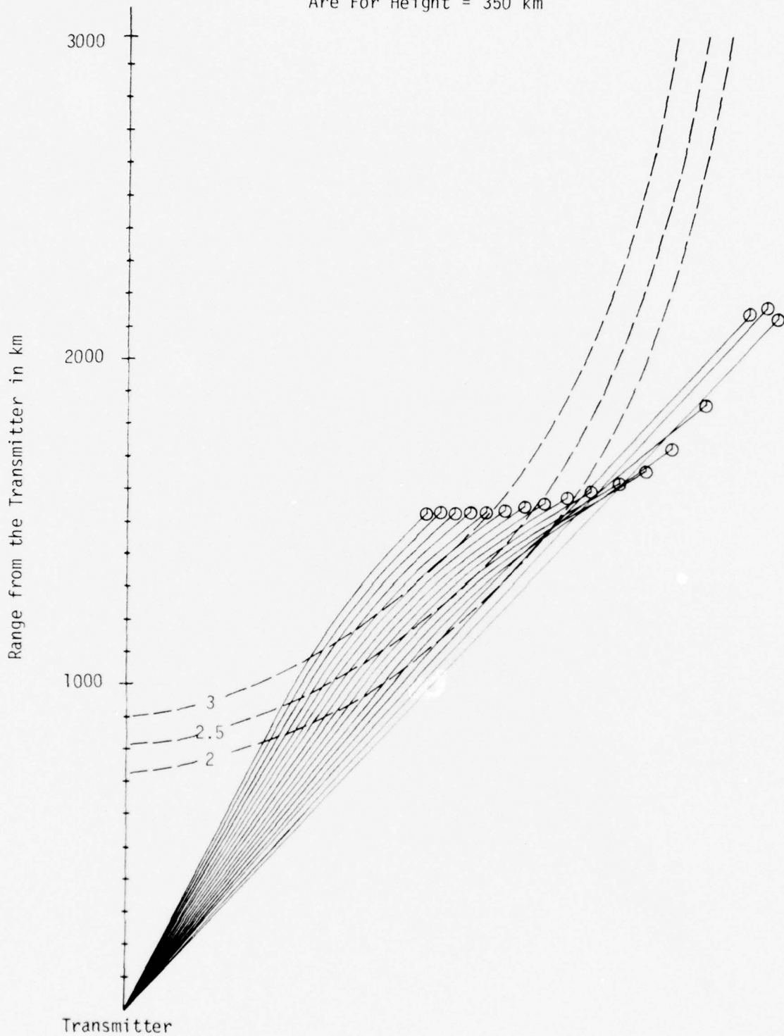
FIGURE 18. RAY PATHS PLOTTED AS A FUNCTION OF RANGE AND AZIMUTH FROM THE TRANSMITTER FOR 7° ELEVATION ANGLE, TRANSMISSION FREQUENCY 5 MHz, AND IONOSPHERIC MODEL TROUGH I
