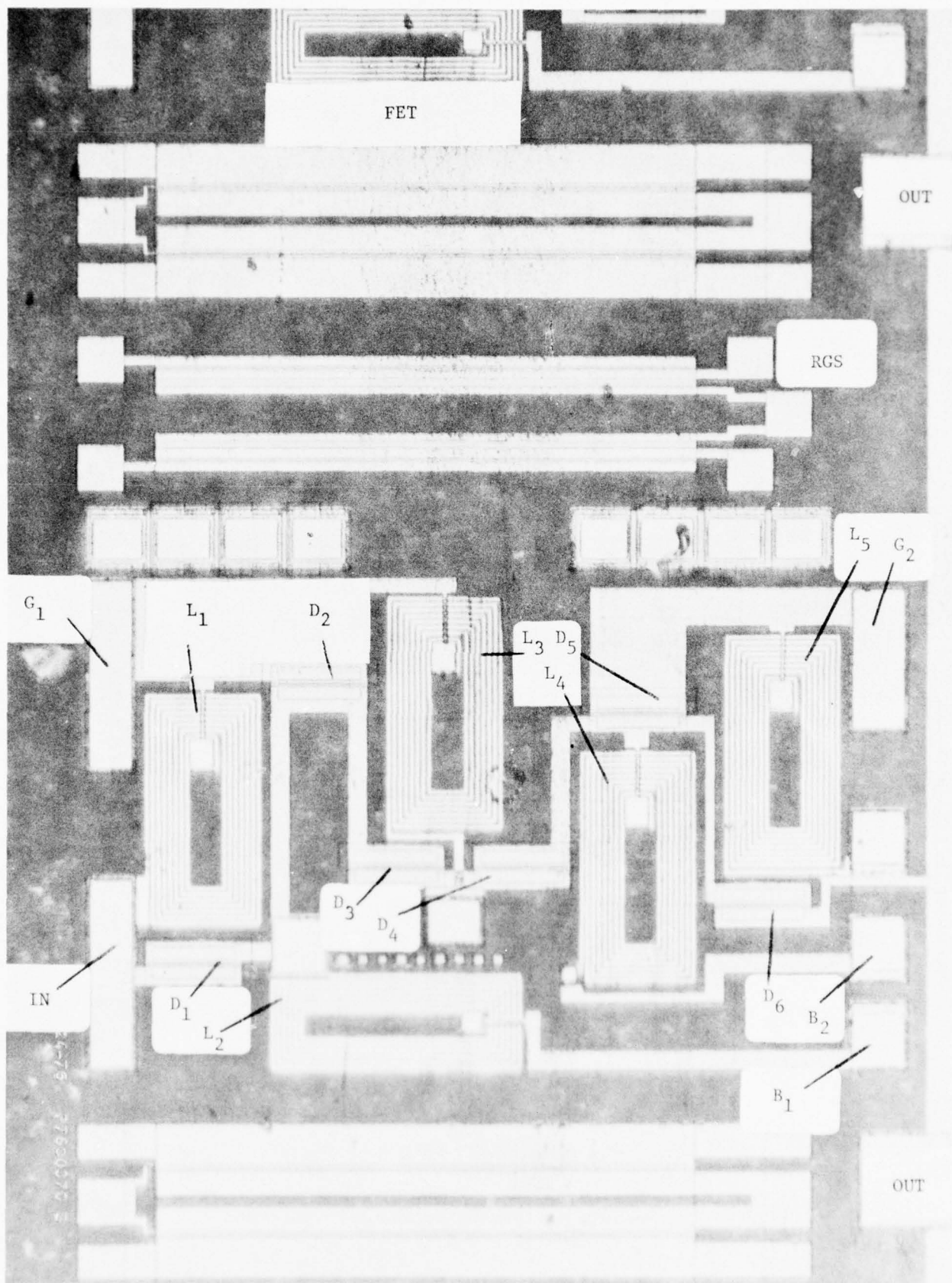
Figure 12. Layout of the Switch
