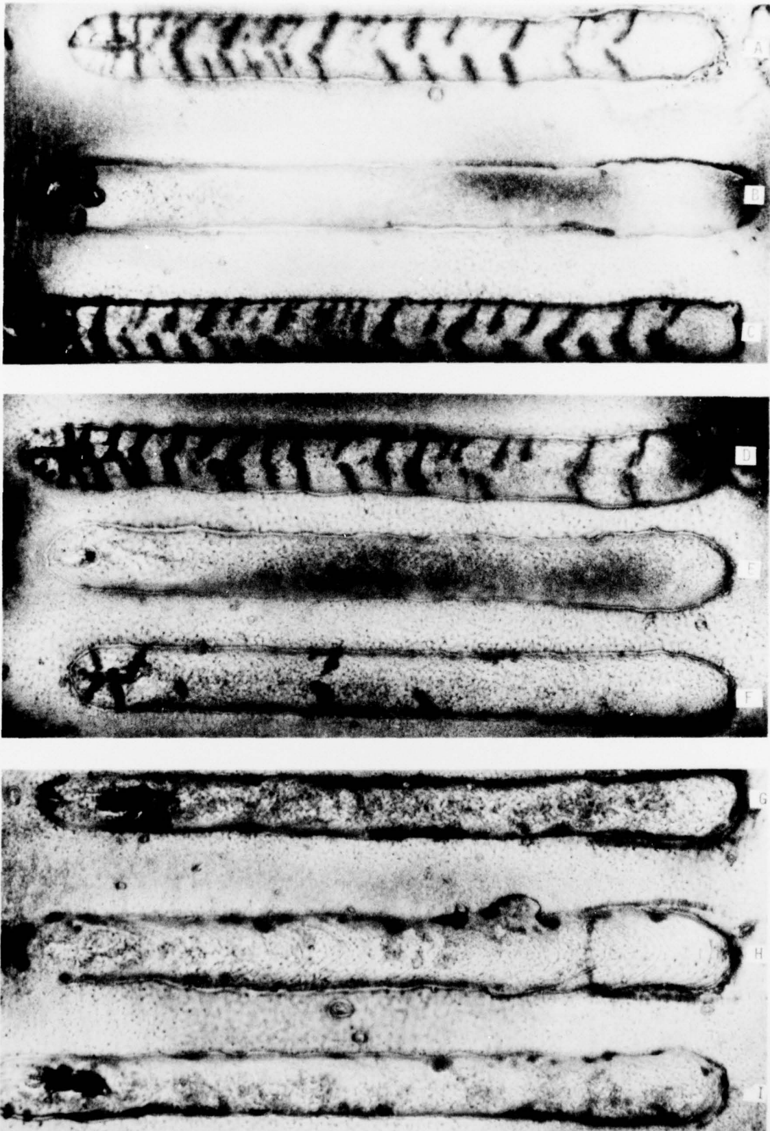
FIGURE 2. HOT CRACKING IN BEADS-ON-PLATE WELDS CONTAINING RARE EARTH ADDITIONS
