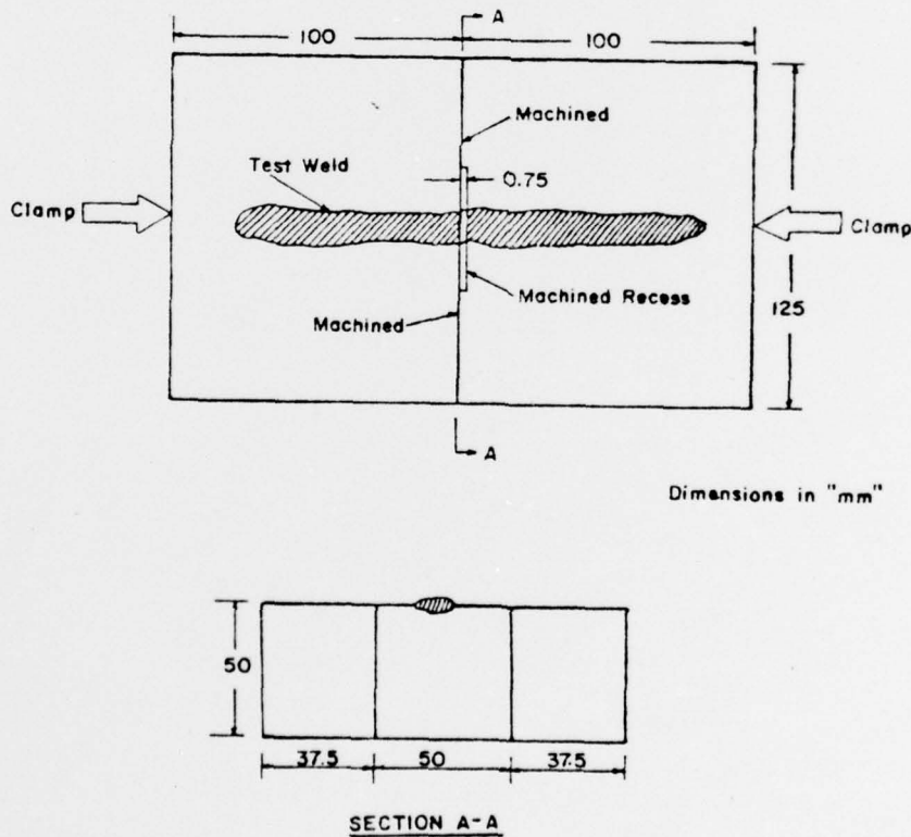
FIGURE 1. STANDARD GBOP (gapped bead-on-plate) (Ref. a)
