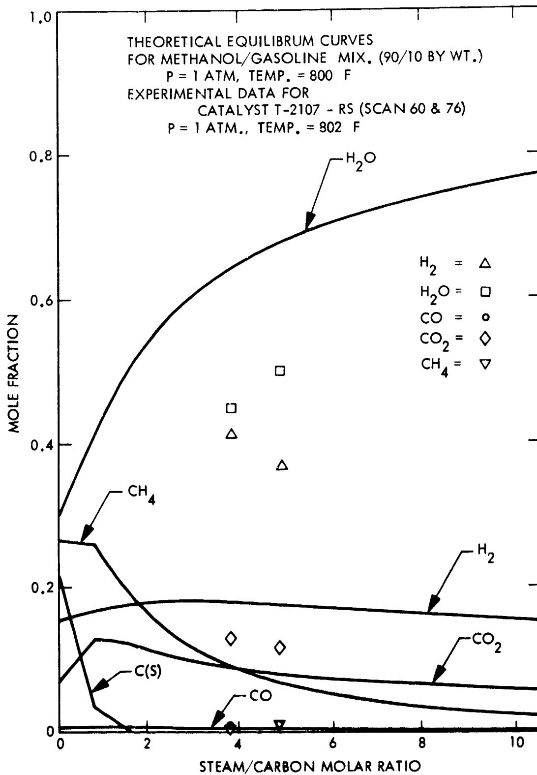
Figure 5-9. Product Distribution
