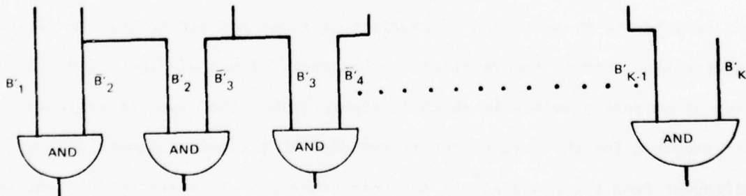
Figure 2-9. Enable Circuit
