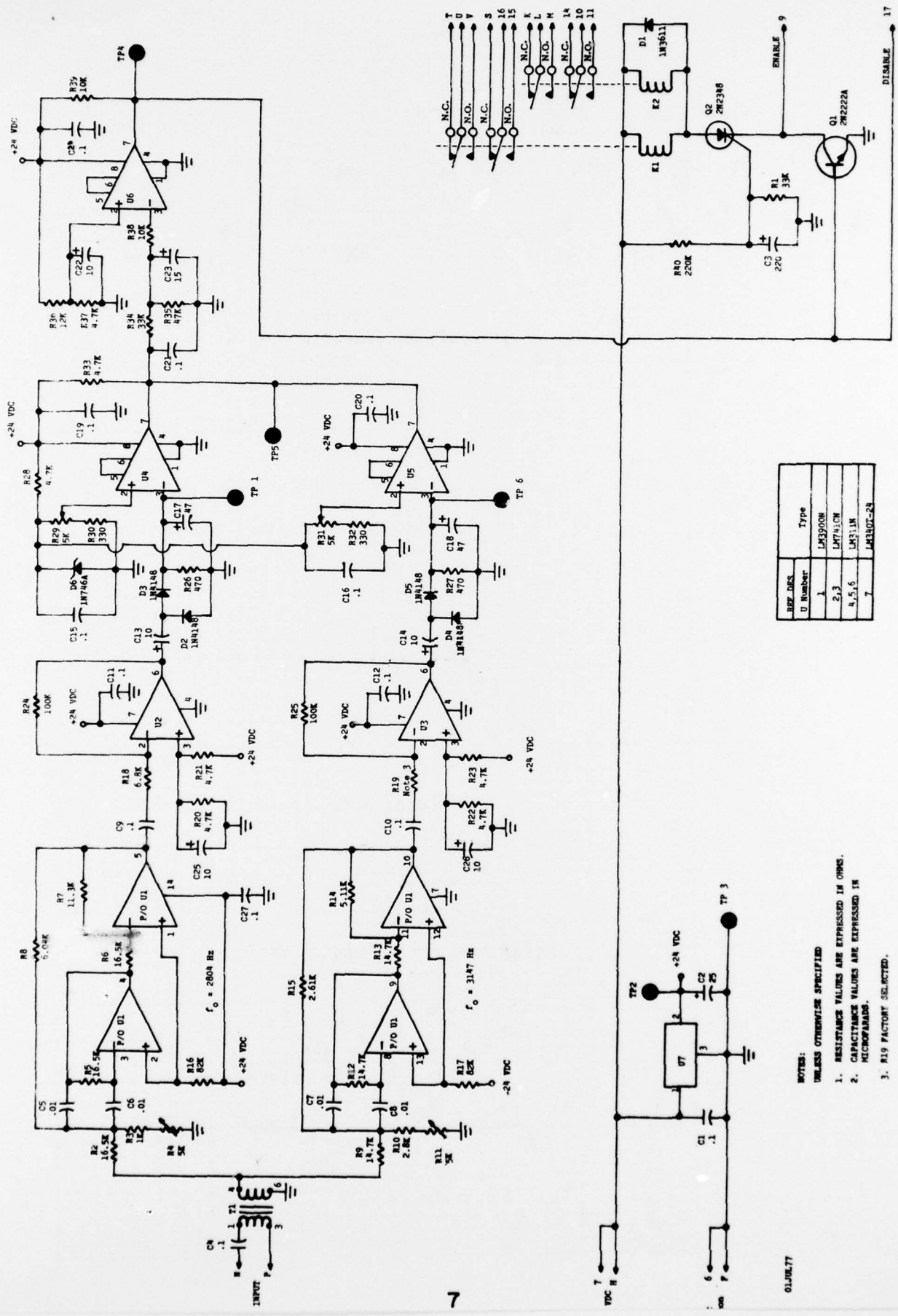
FIGURE 2 MULTITONE DETECTOR SCHEMATIC DIAGRAM
