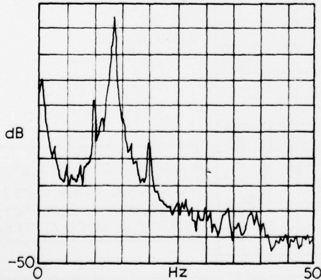
FIG. 11c. WOOD BLOCKS 0.02 dB ref.
