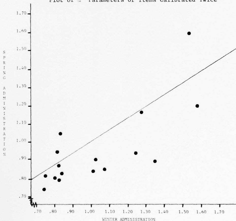
Figure 2 Plot of a Parameters of Items Calibrated Twice
