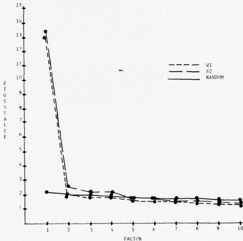
Figure 1 Eigenvalues for W1 data, S2 Data and Comparable Random Data
