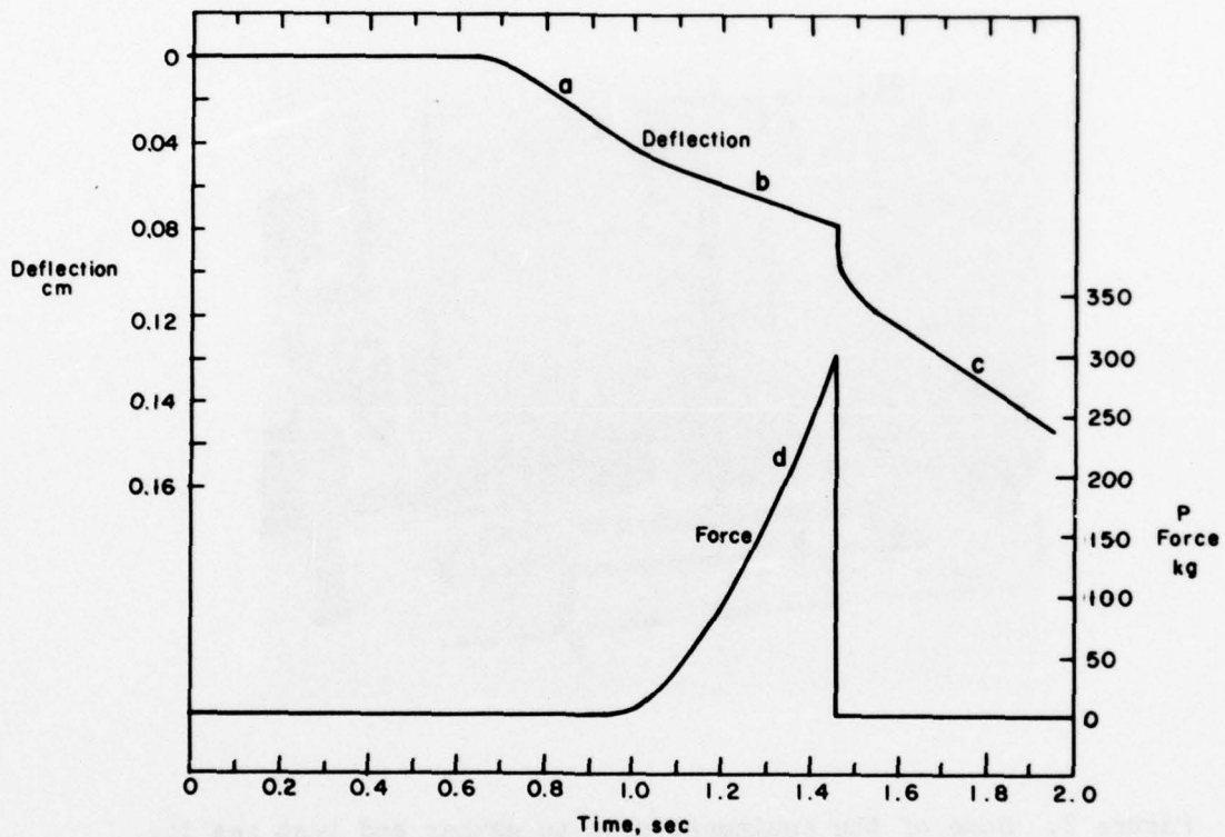
Figure 3. Typical record of a test, specimen 9 of core 3 from drop 6. (Notes: a and c represent ram speed under zero load. Line b represents ram speed during test. Line d represents load build-up with time).
