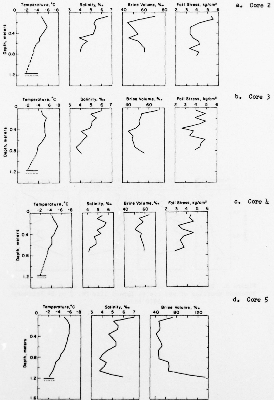
Figure 9. Temperature, salinity, brine volume and Brazil tensile strength profiles of sea ice at Impact Site No. 2 on 27 February 1970.
