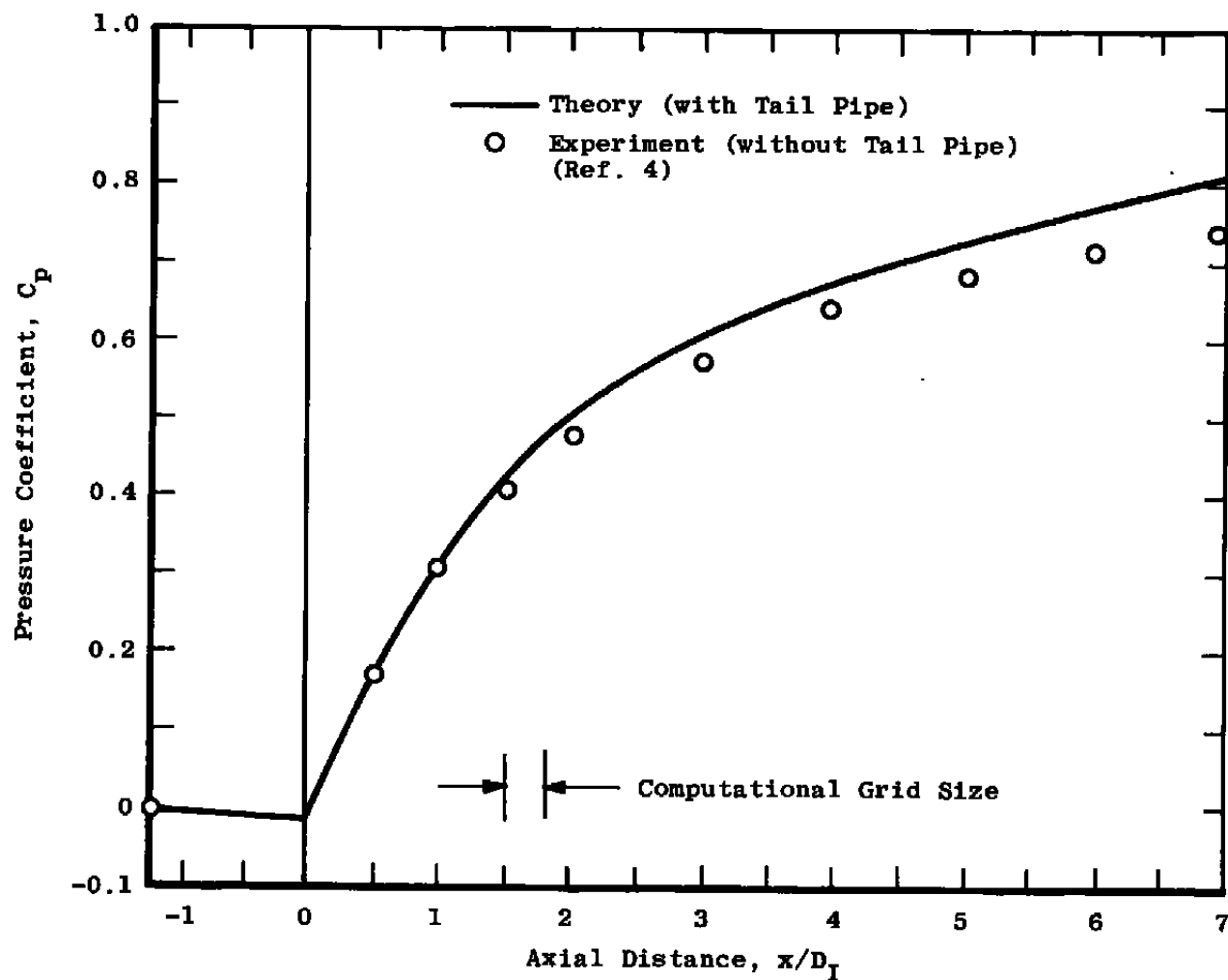
Figure 18. Pressure coefficient in 8-deg conical diffuser with fully developed inlet profile.
