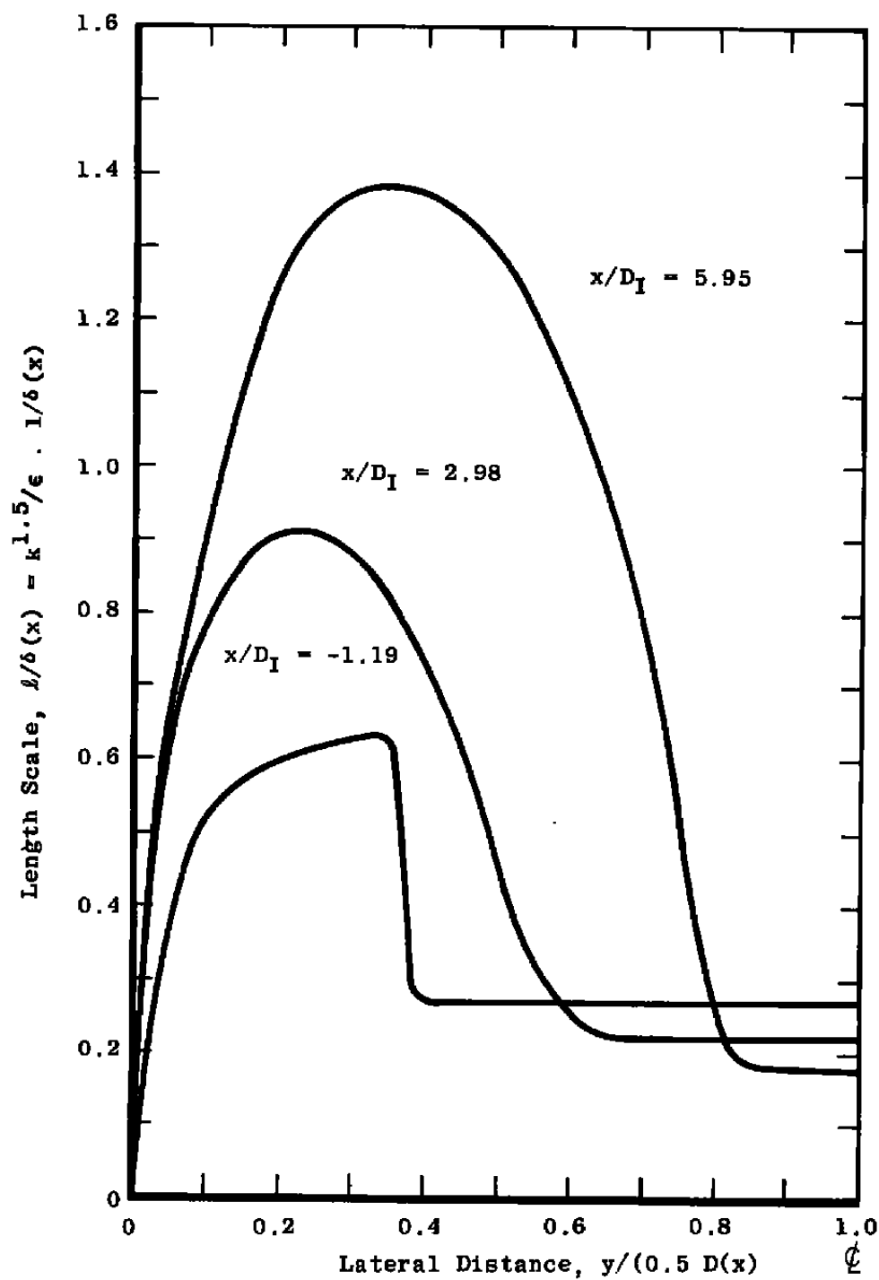
Figure 25. Length scale distributions in 8-deg conical diffuser with a boundary-layer inlet condition, \delta_I = 0.2 D_I .
