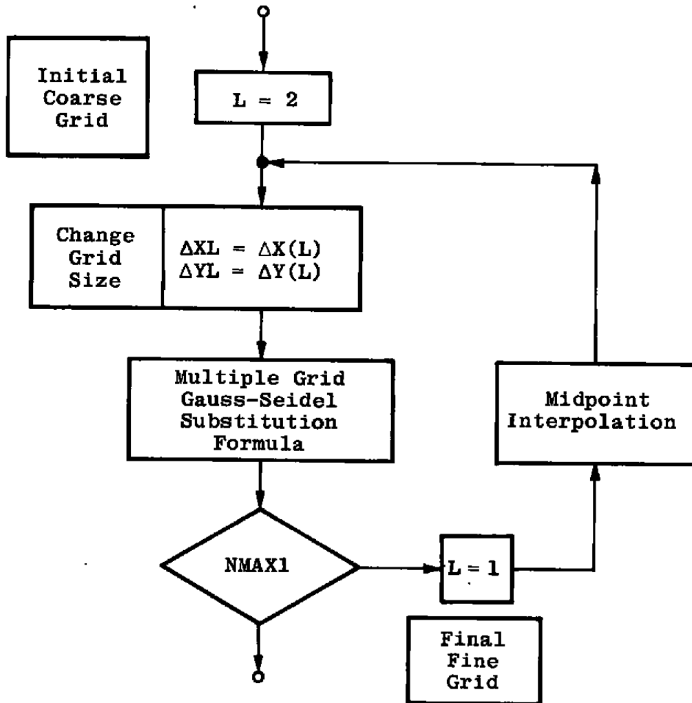
Figure 8. A dual grid Gauss-Seidel iteration scheme.
