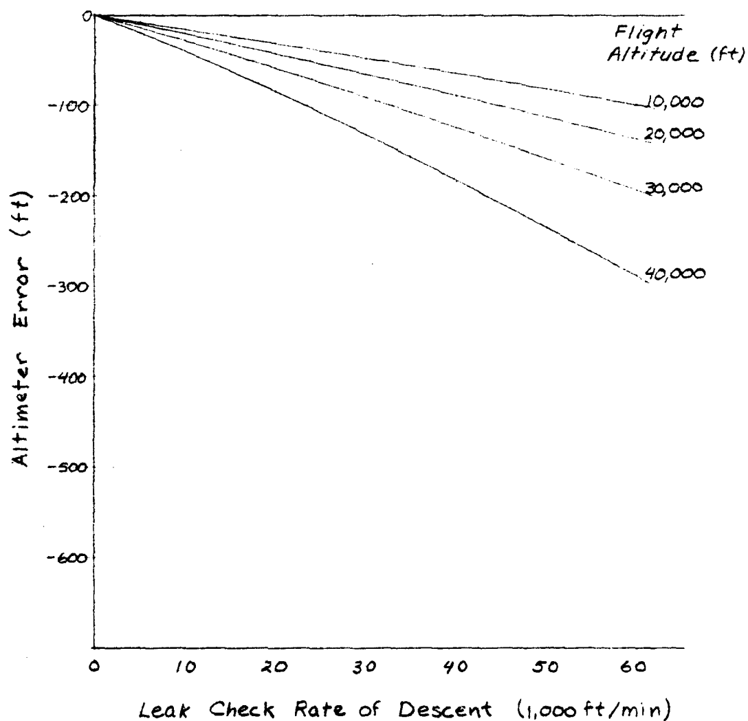
FIGURE C6 EFFECT OF LEAK ON ALTIMETER, AP_2 = 8 in. Hg
