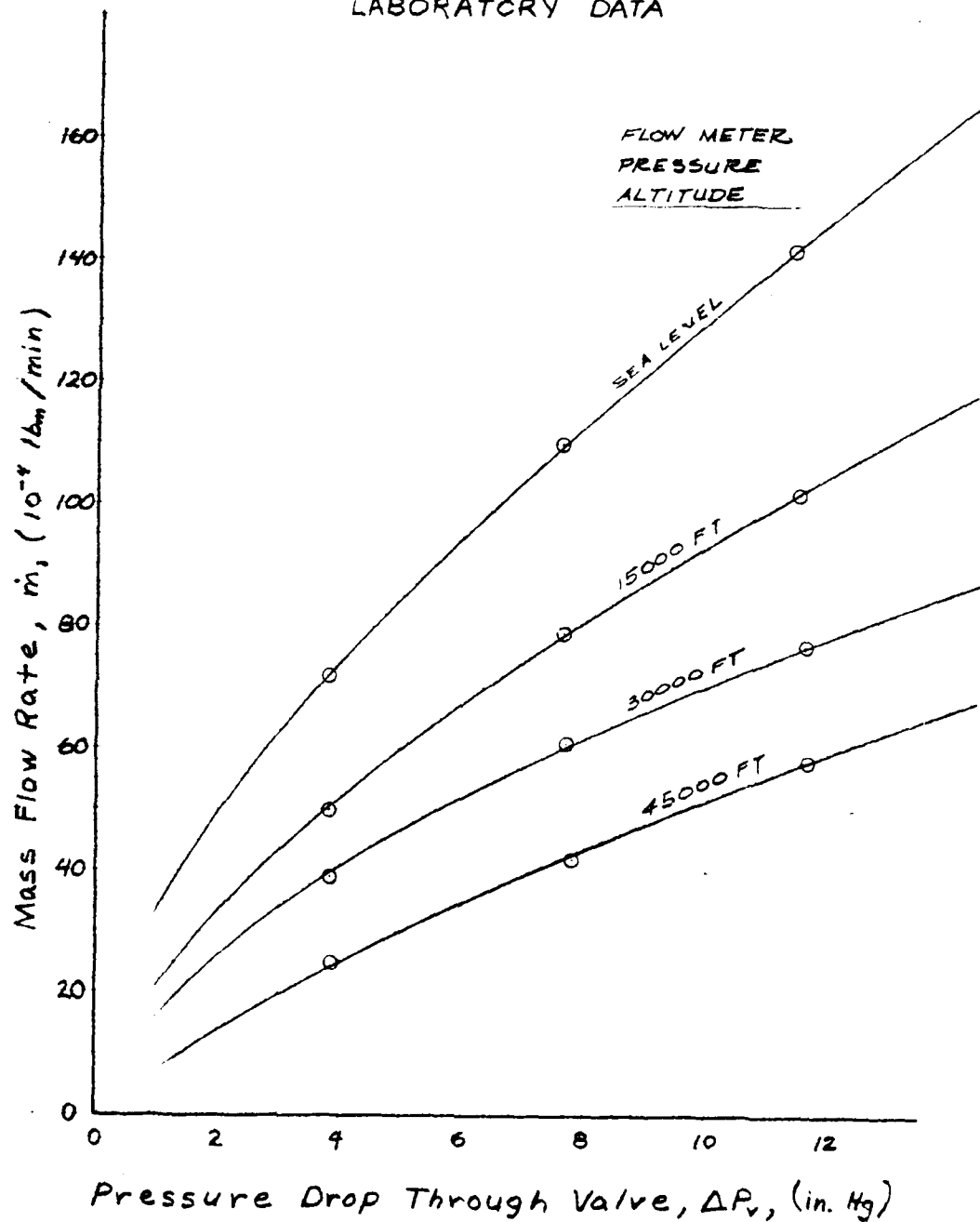
FIGURE A6 MASS FLOW RATE vs VALVE PRESSURE DROP FOR CONSTANT FLOW METER PRESSURE, VALVE SETTING = 1-9
