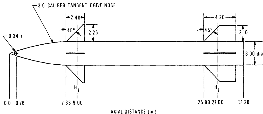
Figure 3. Canard-Control Missile Configuration Dimensions (Body Plus Canard Plus Tail)
