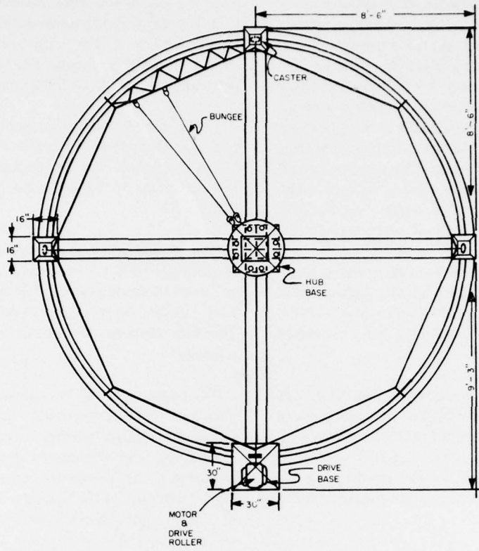
Figure 1. Schematic of turntable equipment.
