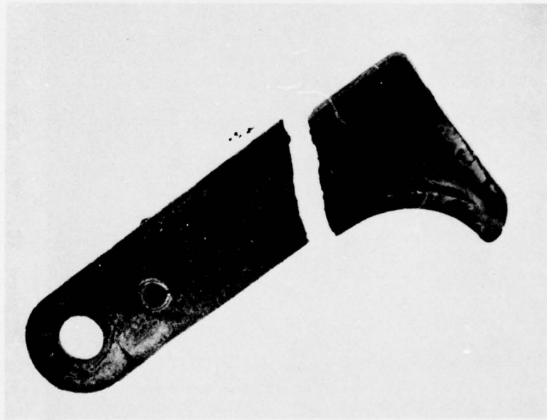
Figure 32. Fractured retaining pin from spring-loaded hitch.
