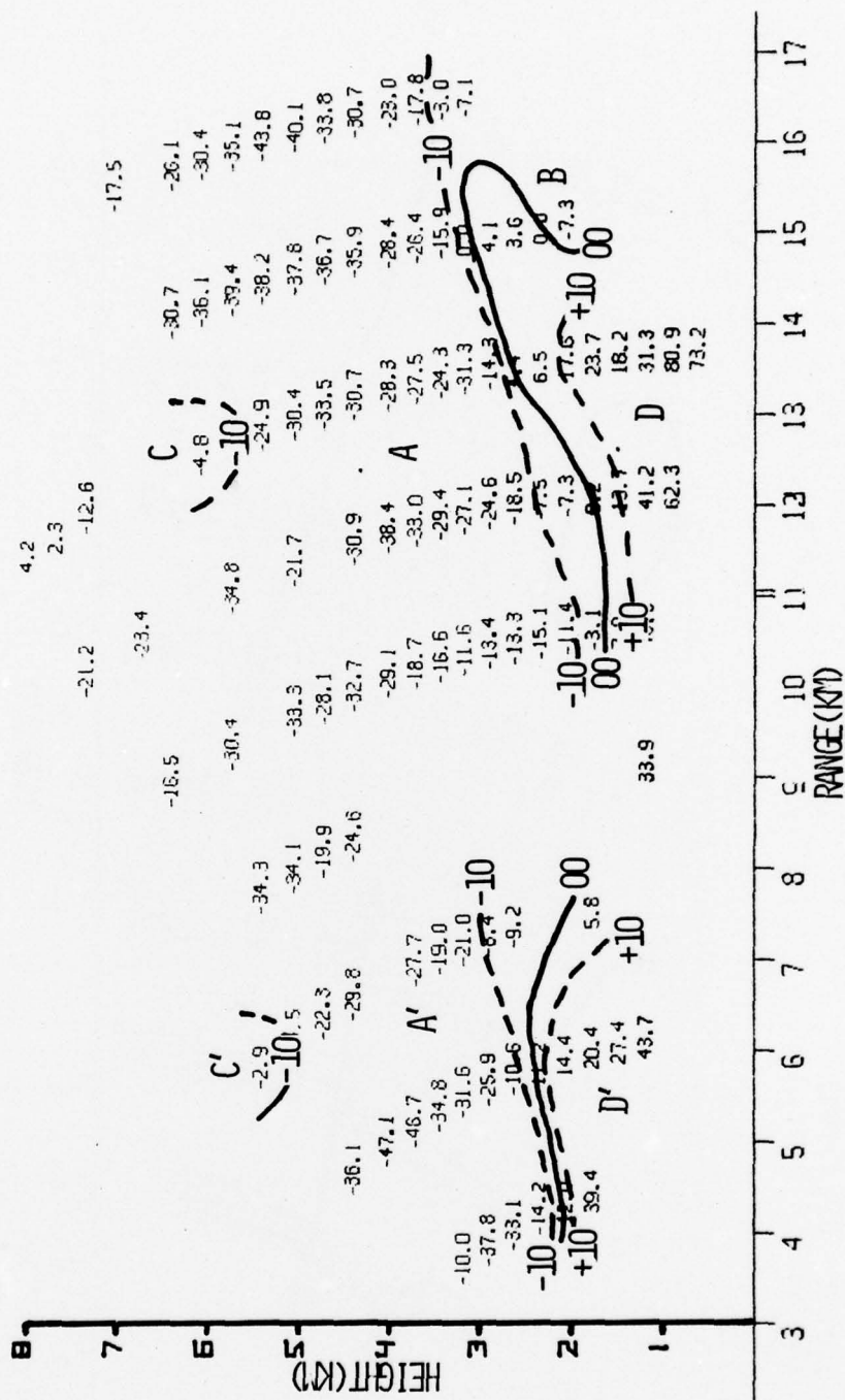
Figure 18 \Delta\theta field for Azimuth 339°, 1758 EDT, 23 June 1974.
