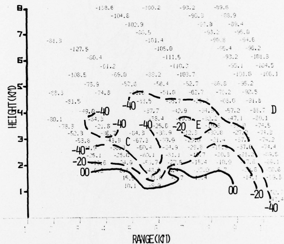
Figure 21 \Delta\theta field for Azimuth 278°, 1808 EDT, 23 June 1974.
