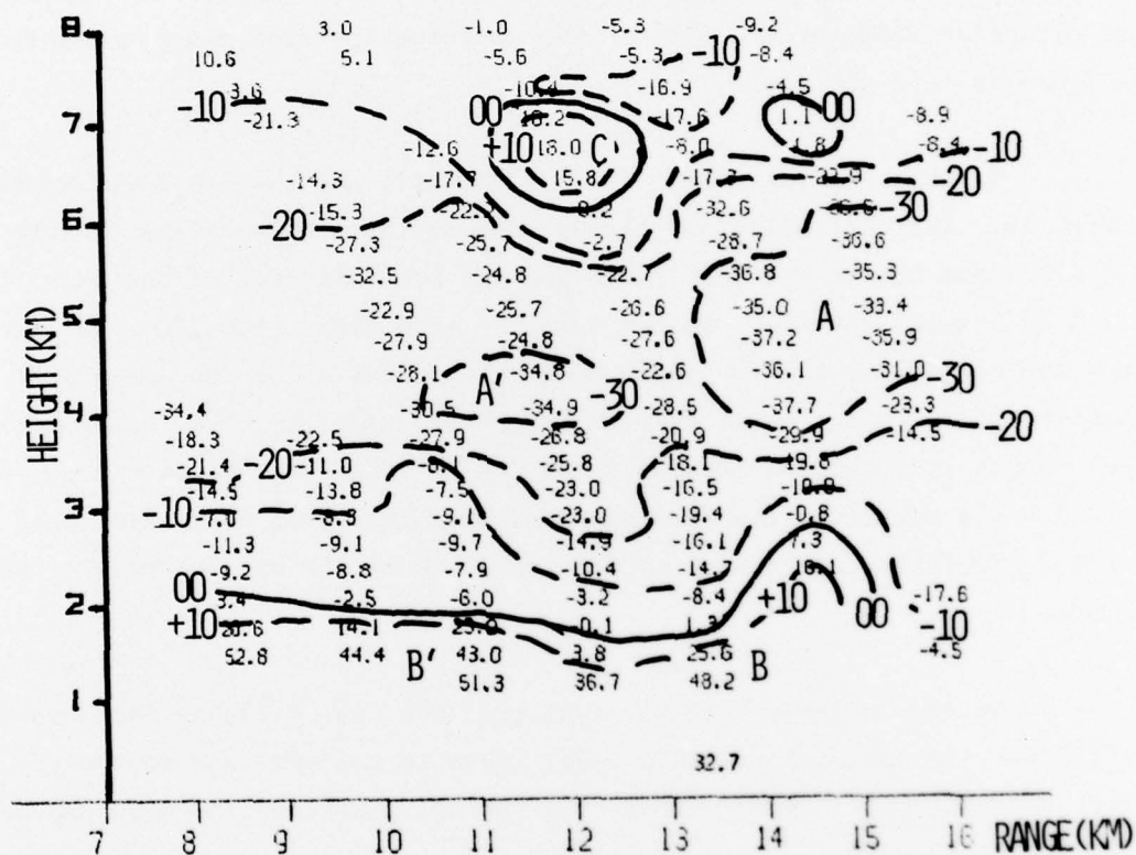
Figure 19 \Delta\theta field for Azimuth 330°, 1756 EDT, 23 June 1974.
