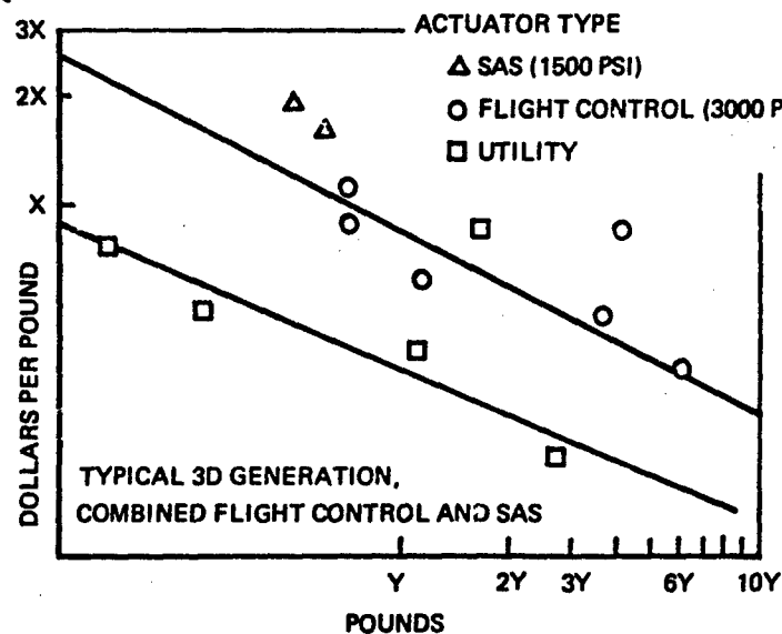
Figure 9. Acquisition Cost of Hydraulic Actuators.
