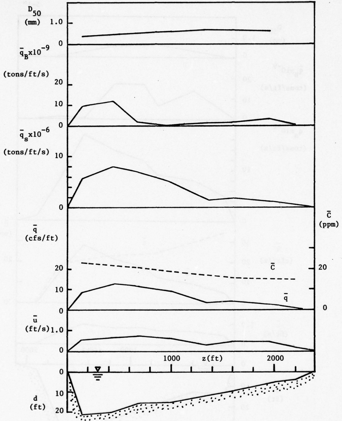
Figure 31. Lateral distributions of d , \bar{u} , \bar{q} , \bar{q}_s , \bar{q}_B , and D_{50} for Sec. 4-1"
