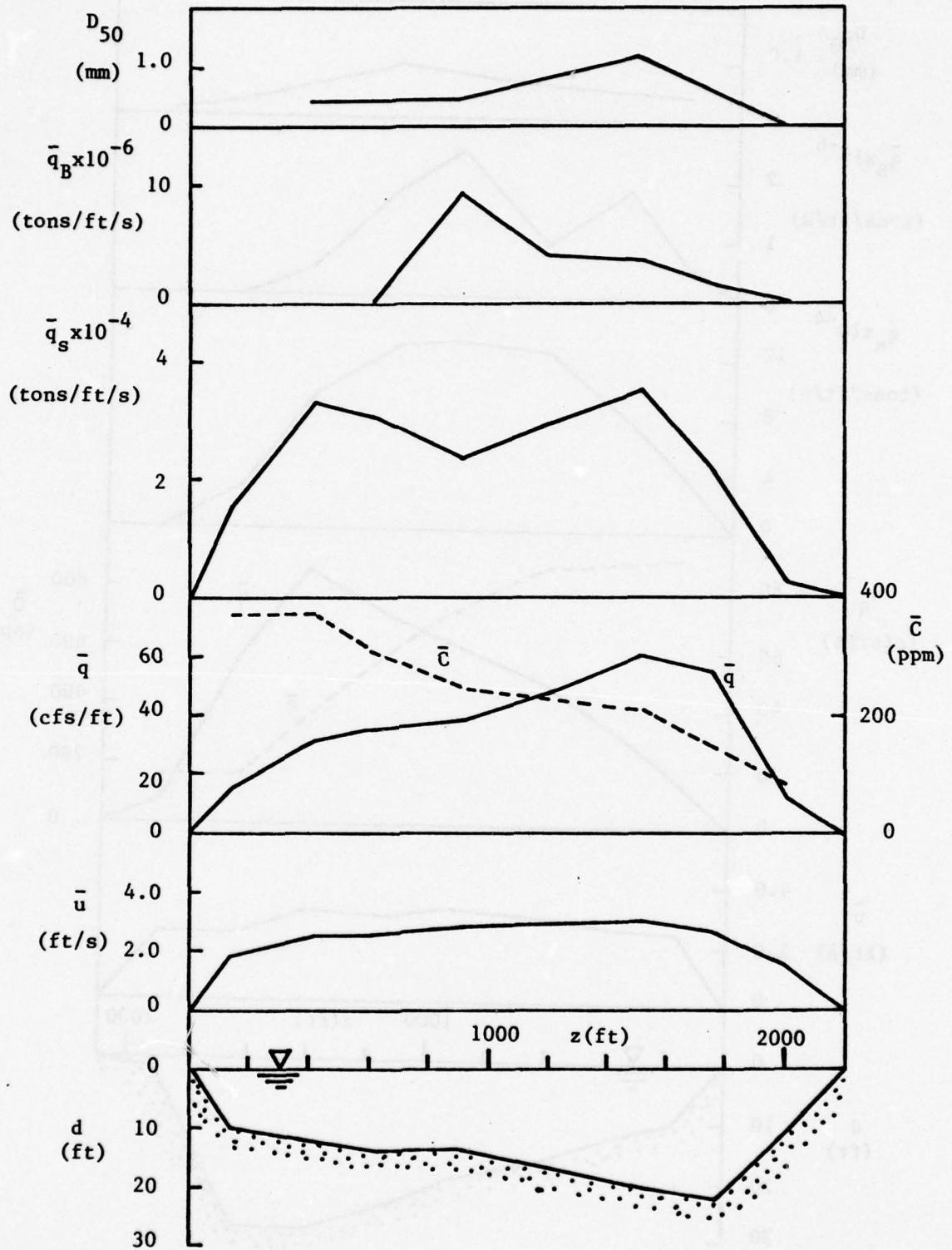
Figure 17. Lateral distributions of d , \bar{u} , \bar{q} , \bar{q}_s , \bar{q}_B , and D_{50} for Sec. 6-1
