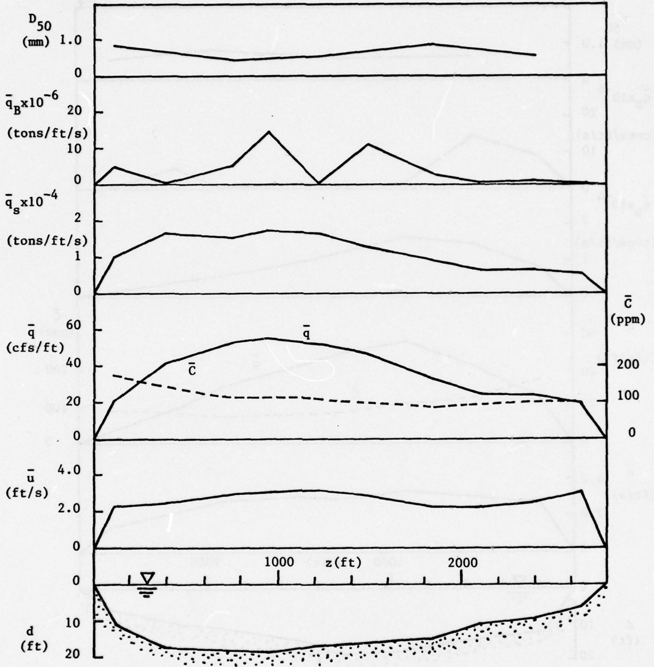
Figure 13. Lateral distributions of d , \bar{u} , \bar{q} , \bar{q}_s , \bar{q}_B , and D_{50} for Sec. 2-1
