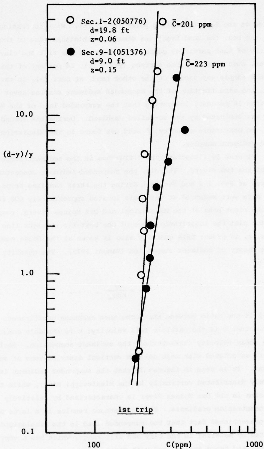
Figure 39. Typical vertical distributions of suspended-sediment concentration obtained at Sec. 1-2 and Sec. 9-1 (1st trip)
