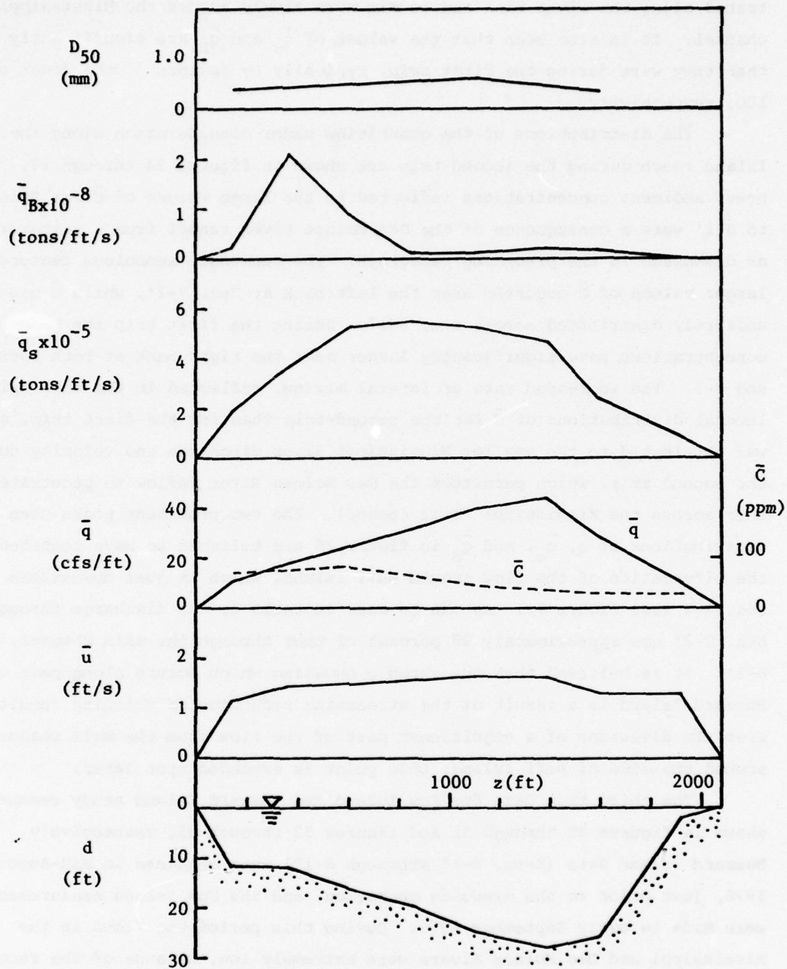
Figure 24. Lateral distributions of d , \bar{u} , \bar{q} , \bar{q}_s , \bar{q}_B , and D_{50} for Sec. 5-1'
