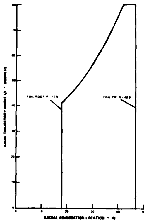
Figure 19 Fan Forward Containment – Axial Trajectory Angle vs. Radial Reingestion Location for Impact at 30 Degrees Forward of the Fan Rotor Plane
