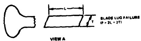
Figure 2 Fan Containment - Single Blade Failure
