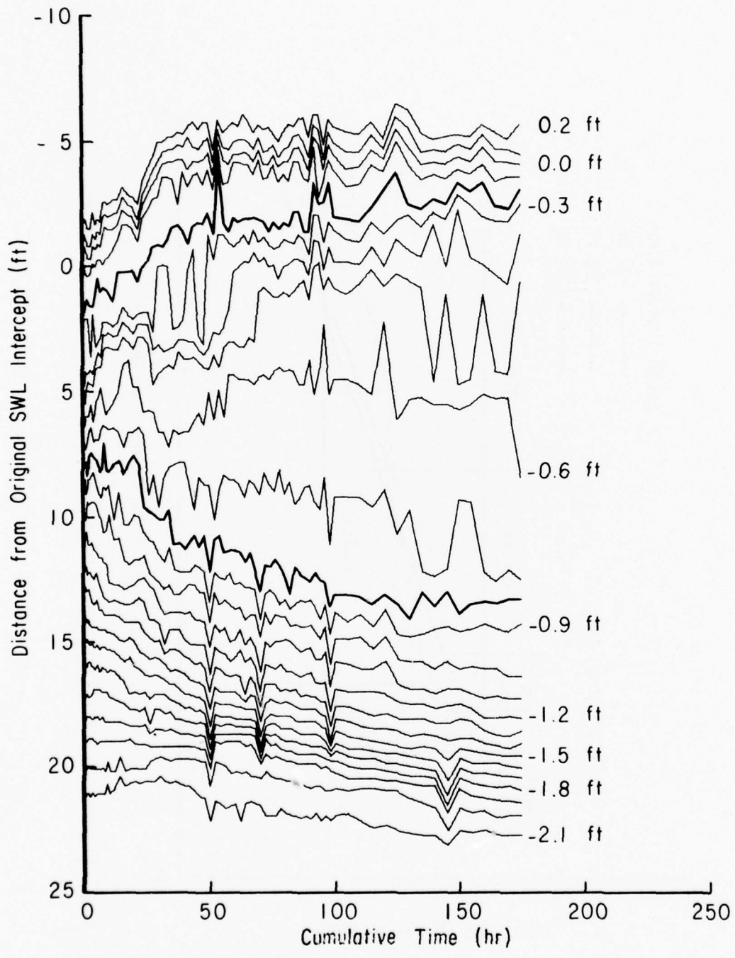
Figure 10. Profile changes along range 1, experiment 70X-06.
