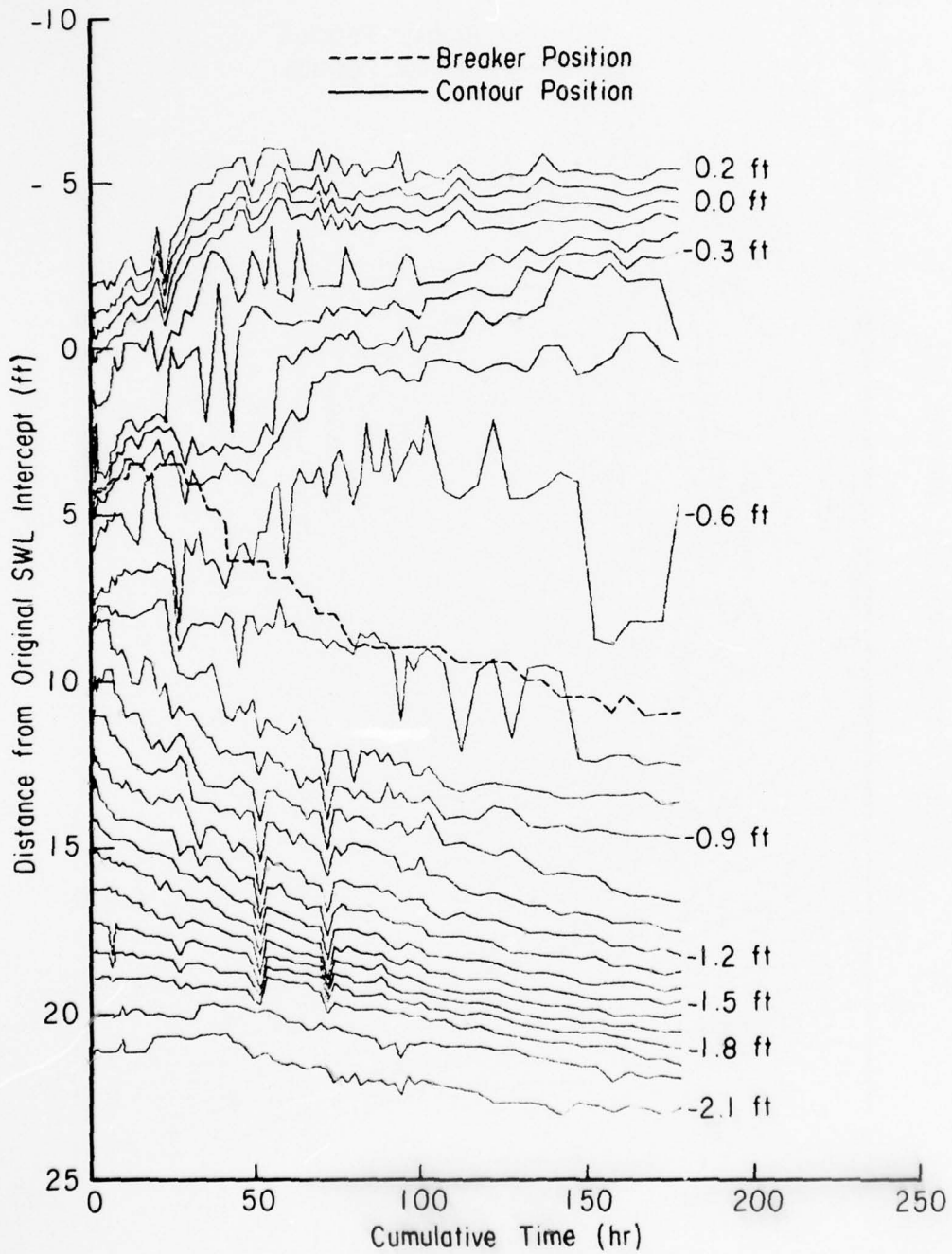
Figure 34. Movement of the breaker position in experiment 70X-06.
