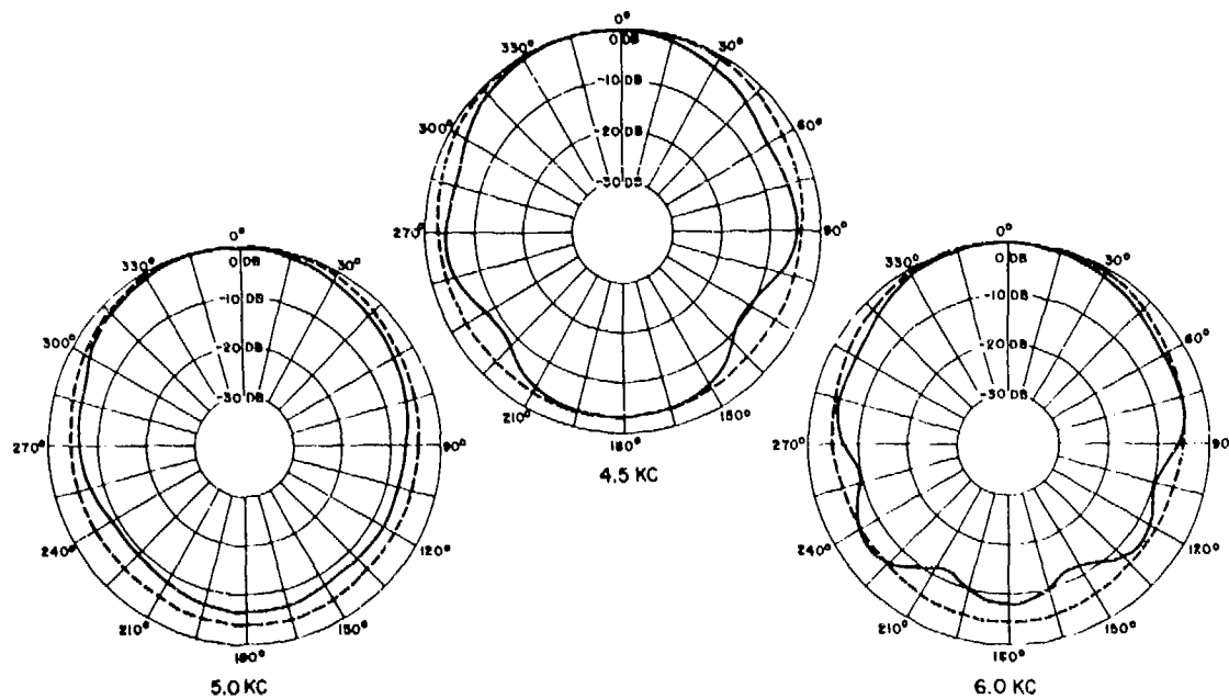
Fig. 11. Comparison of directivity; solid line represents measured directivity of cavity resonator with 1\frac{1}{2} -inch-deep cavity at end of tube; dashed line represents theoretical directivity of plane piston at end of tube.
