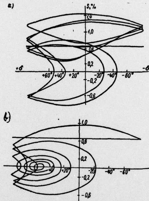
Fig. 3. Phase trajectories of the synchronization process:
