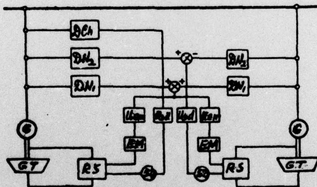
Fig. 1. Block diagram of a gas turbogenerator automatic frequency regulator.
