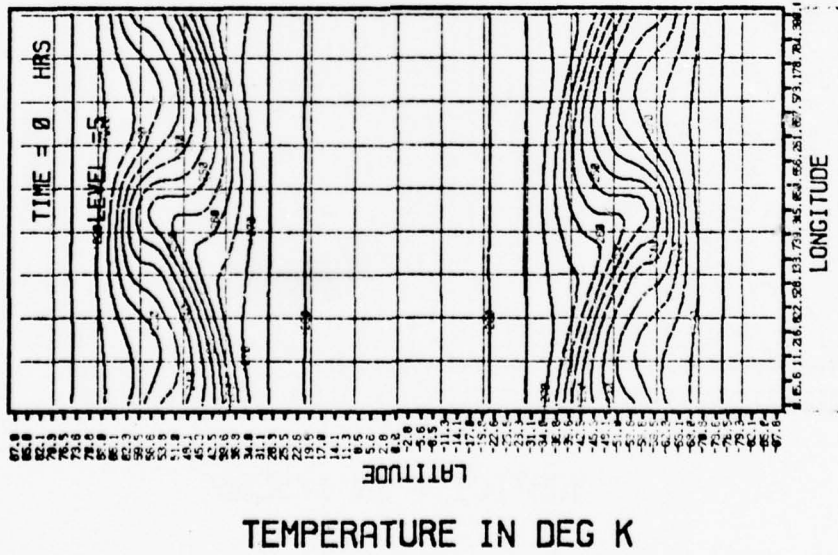
Figure 8. Initial high resolution temperature for \sigma = .9 . Contour interval is 5^{\circ}\text{K} .
