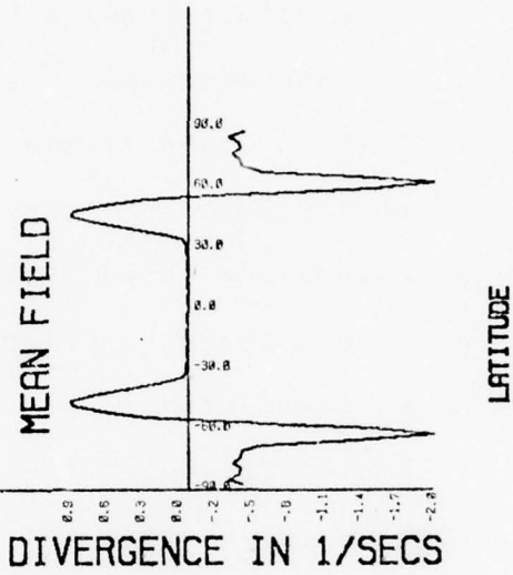
Figure 23. Quasi-geostrophic divergence (high resolution) for \sigma = .9 . Contour interval is 1 \times 10^{-6} \text{sec}^{-1} . Mean field is scaled by 106.
