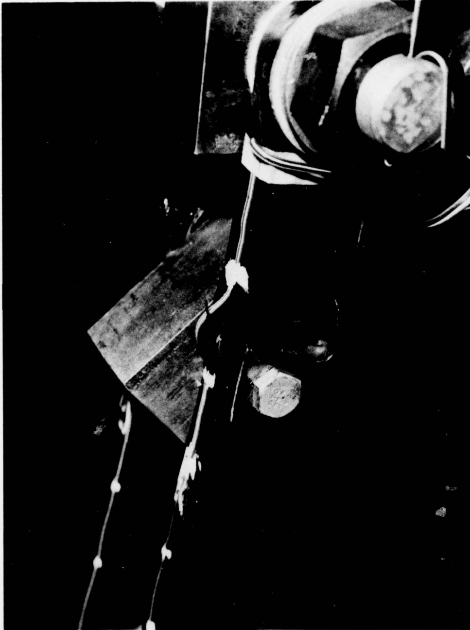
Figure 16. Failed S/N 1 Upper Members After 25% Increased Load (6 Lifetimes on Upper Members)
