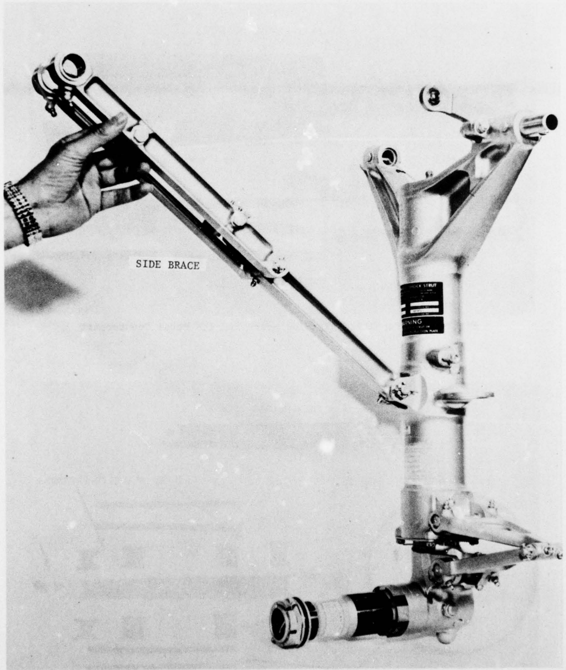
Figure 2. Side Brace Locks Main Landing Gear Down
