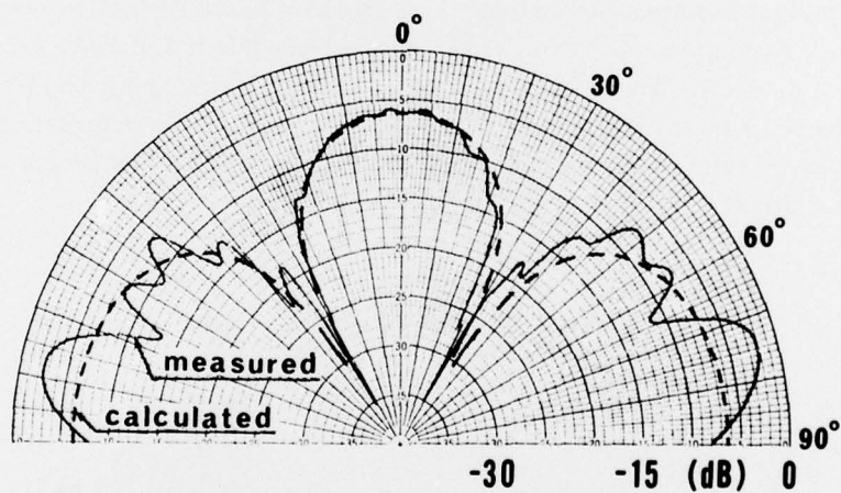
Figure 6. Radiation Pattern Along the E-plane of the Third Mode, 9.15 GHz
