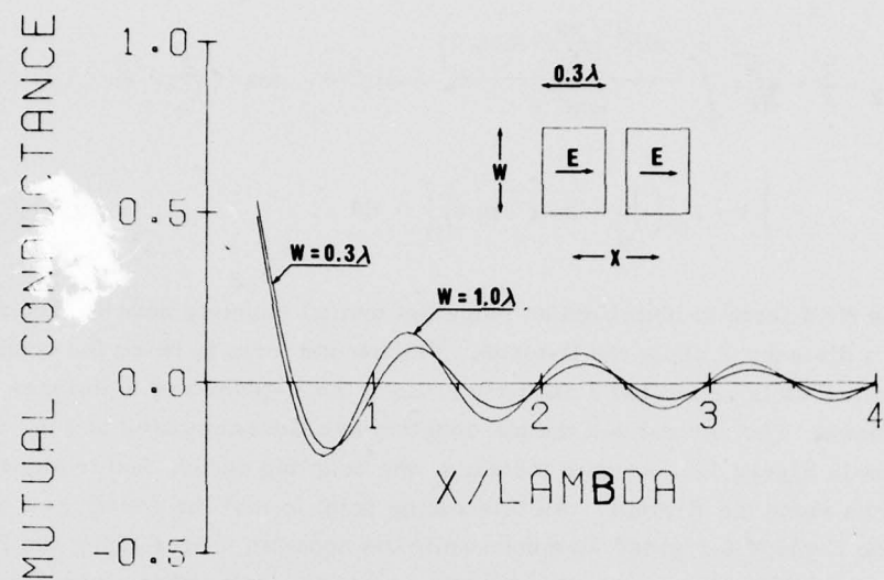
Figure 11. Normalized Mutual Conductance Between Two Rectangular Microstrip Elements Along the E-plane
