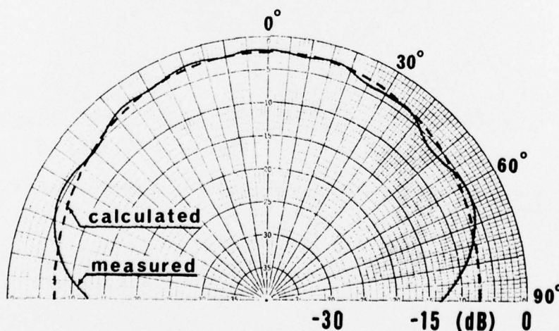
Figure 4. Radiation Pattern Along the E-plane of the First Mode, 3.10 GHz
