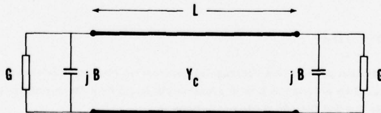
Figure 3. Network Model of the Microstrip Radiating Element
