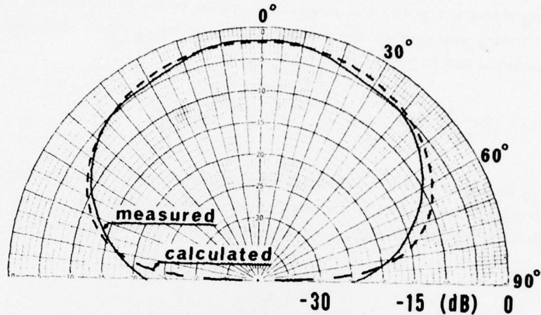
Figure 7. Radiation Pattern Along the H-plane of the First Mode, 3.10 GHz
