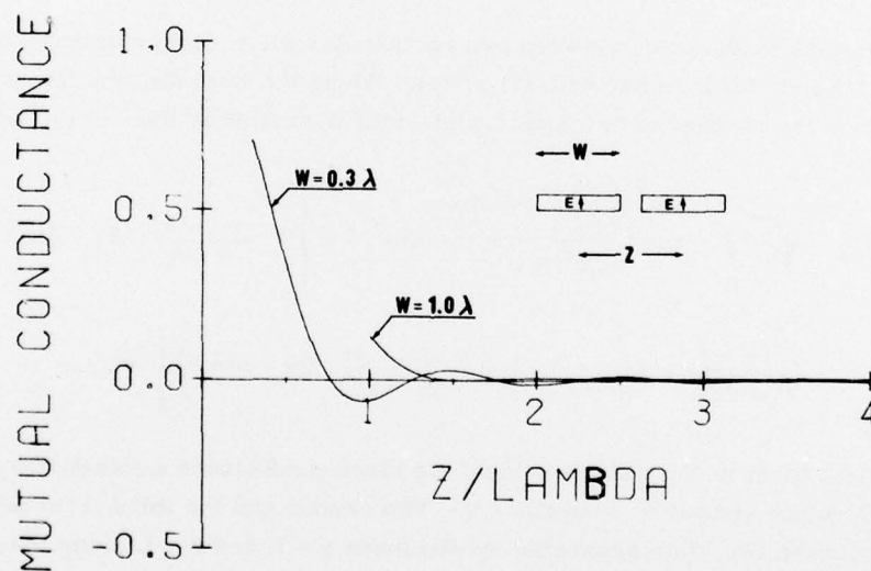
Figure 10. Normalized Mutual Conductance Between Two Narrow Slots Along the H-plane
