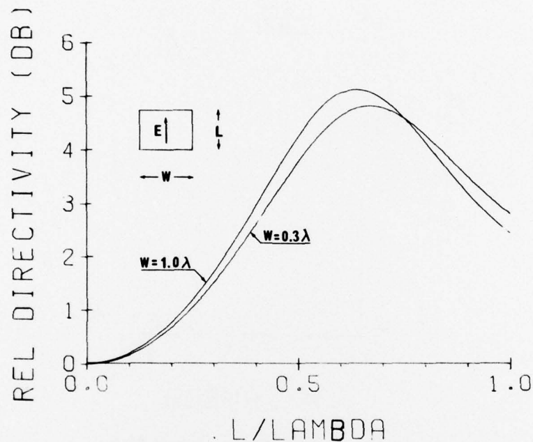
Figure 14. Relative Directivity of a Rectangular Microstrip Element at Resonance
