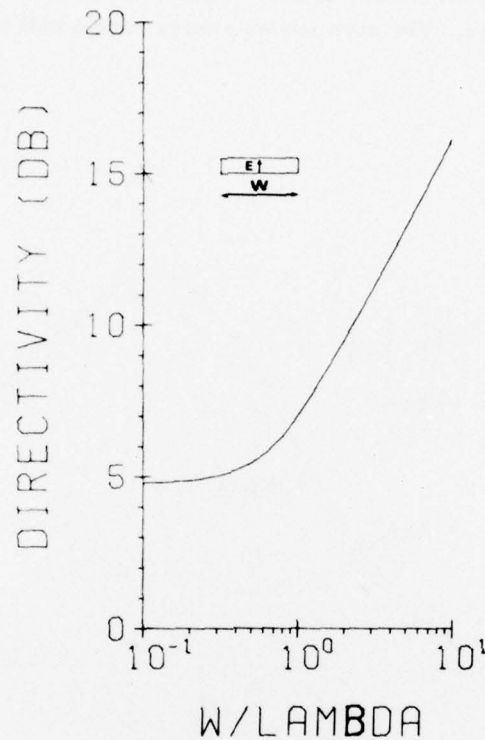
Figure 13. Directivity of a Narrow Slot With Uniform Field Distribution
