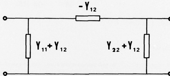
Figure 8. Network Representation of a Pair of Coupled Antennas
