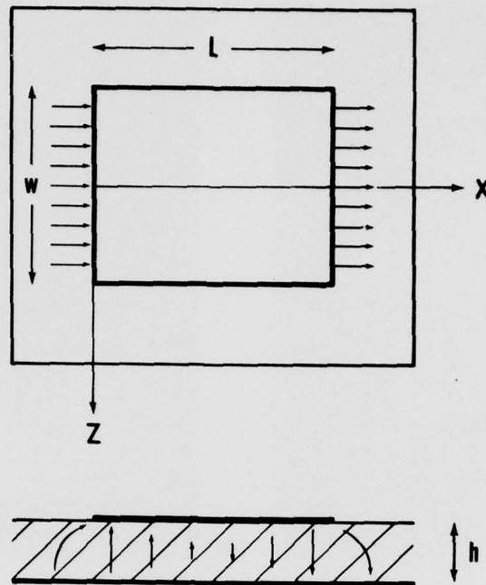
Figure 1. Rectangular Microstrip Radiating Element
