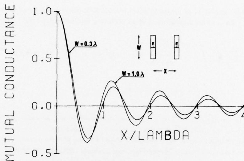
Figure 9. Normalized Mutual Conductance Between Two Narrow Slots Along the E-plane
