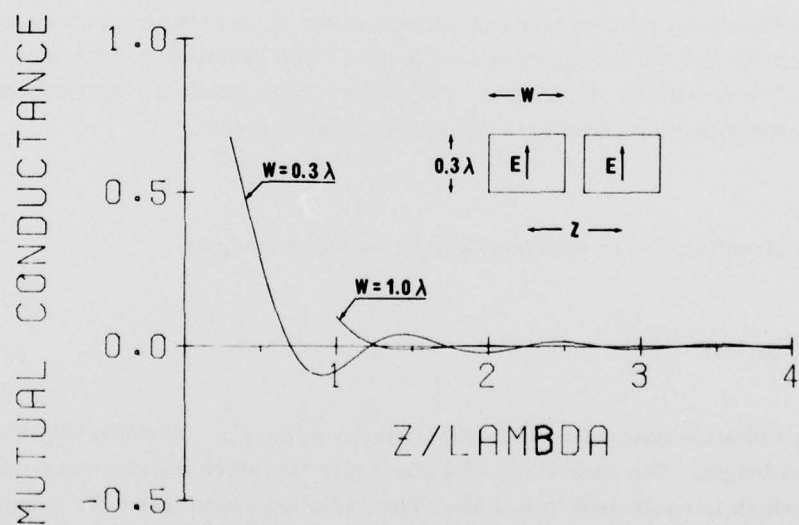
Figure 12. Normalized Mutual Conductance Between Two Rectangular Microstrip Elements Along the H-plane
