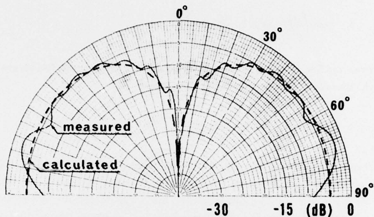
Figure 5. Radiation Pattern Along the E-plane of the Second Mode, 6.15 GHz
