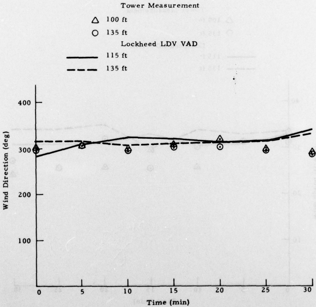
Fig. 6-4 - Comparison of Meteorological Tower Wind Direction Measurements with Lockheed-Huntsville LDV at JFK on 11/5/75 14:06 - 14:36
