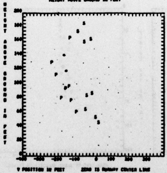
Fig. 5-1 - Wake Vortex Trajectory of B-747 Aircraft - Date, 10/31/75; Time, 16:51:30
