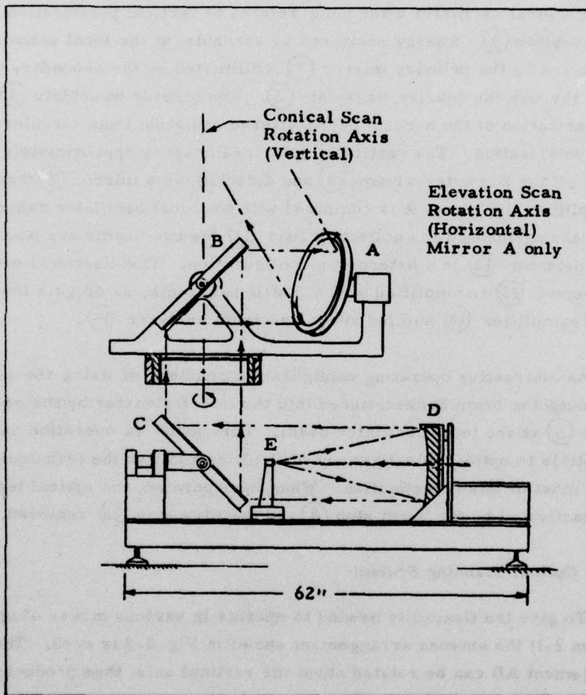
Fig. 2-3 - Scan Equipment Added to LDV
