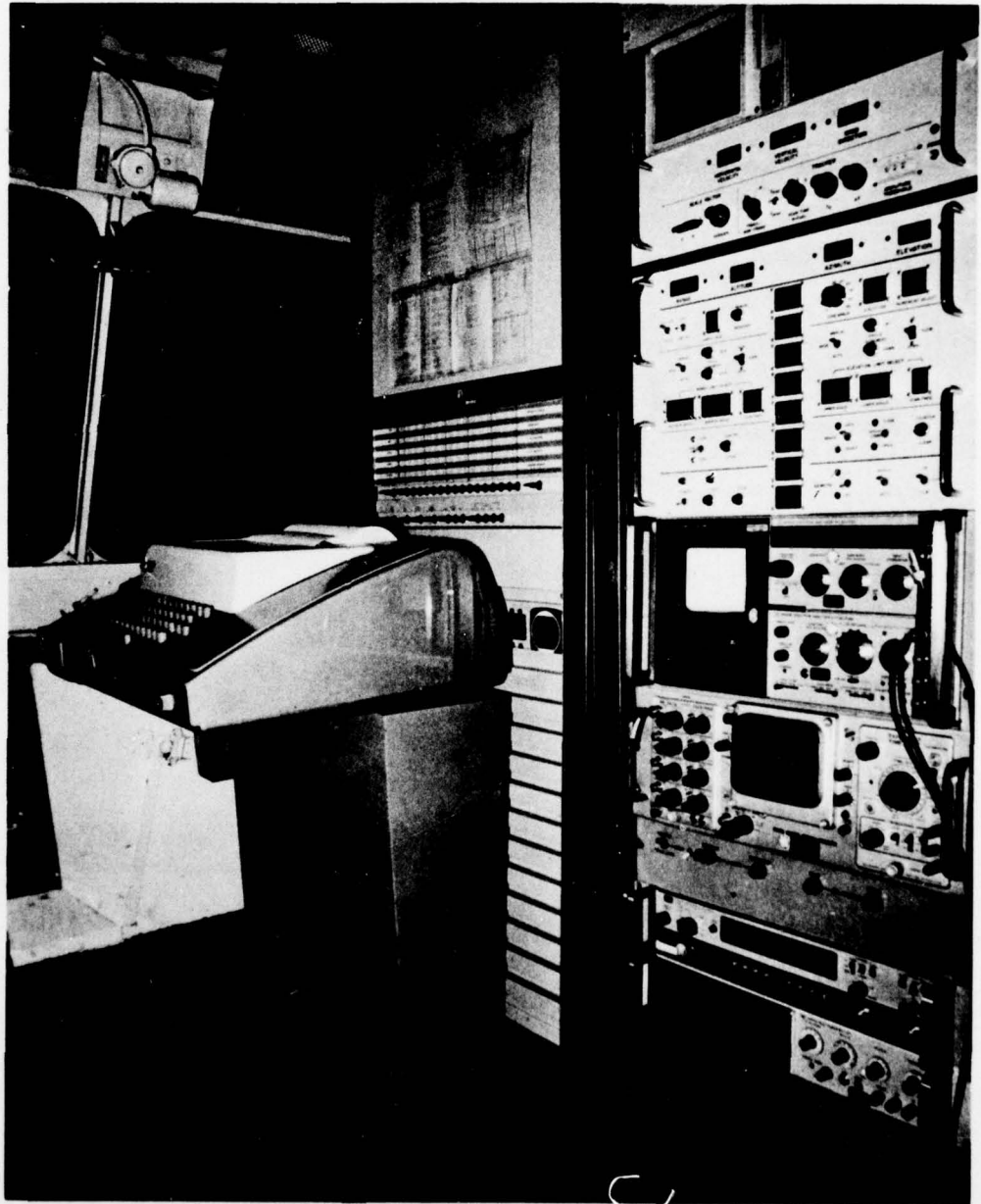
Fig. 2-12 - Computer Mainframe, Teletype, and LDV Electronics
