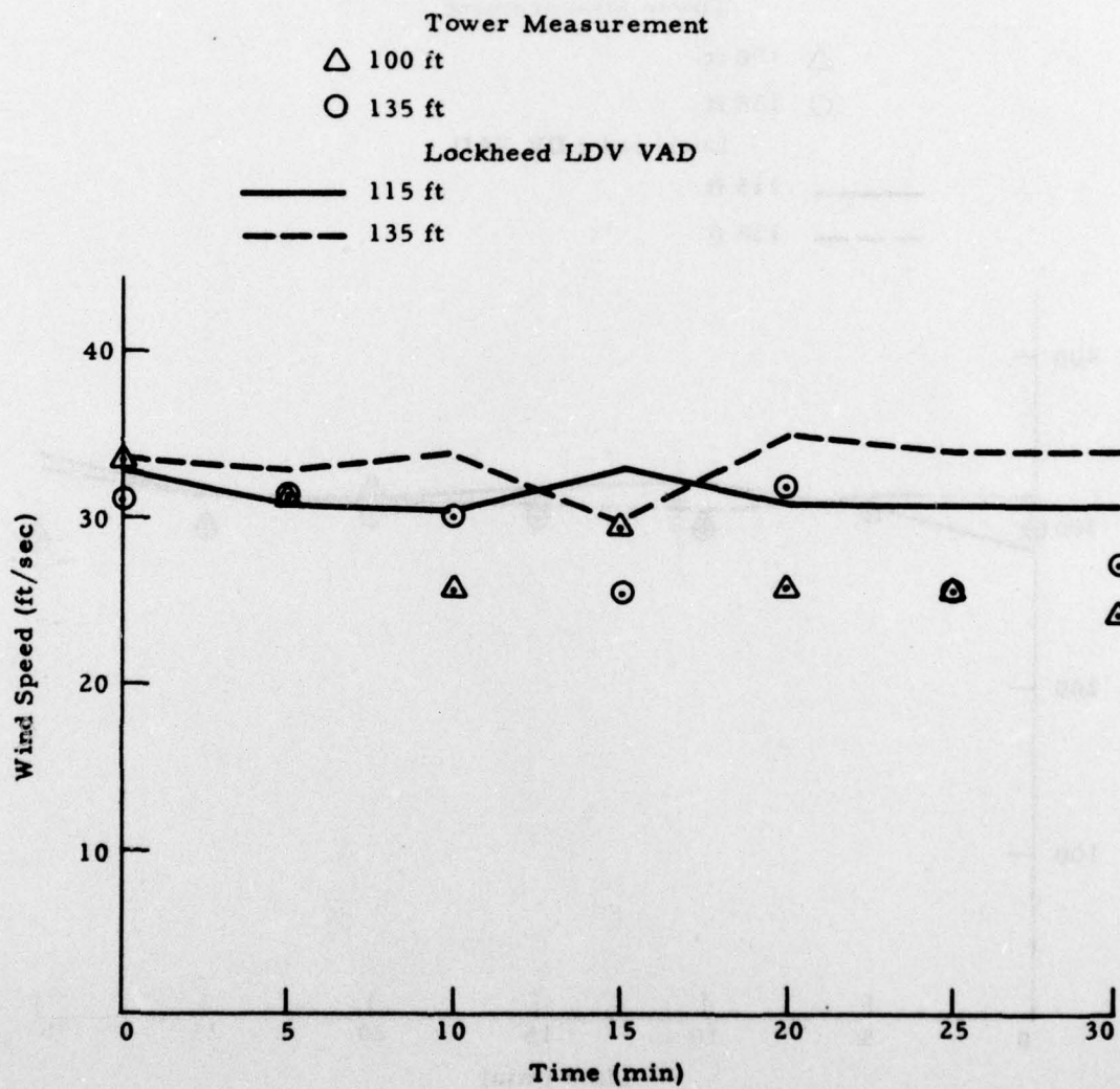
Fig.6-3 - Comparison of Meteorological Tower Wind Speed Measurements with Lockheed-Huntsville LDV at JFK on 11/5/75 14:06-14:36
