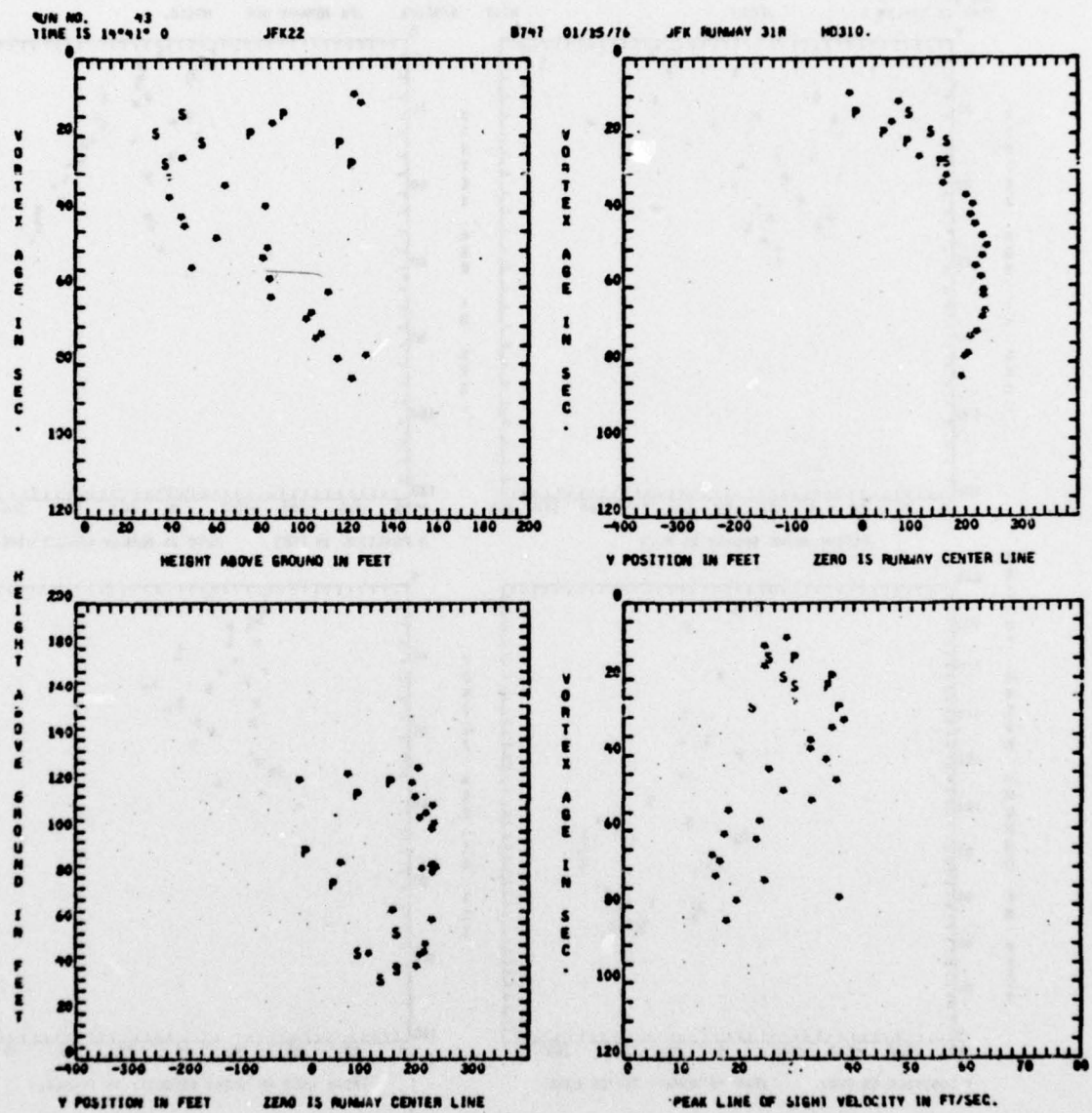
Fig.5-7 - Wake Vortex Trajectory of B-747 Aircraft - Date 1/15/76; Time, 14:41:00
