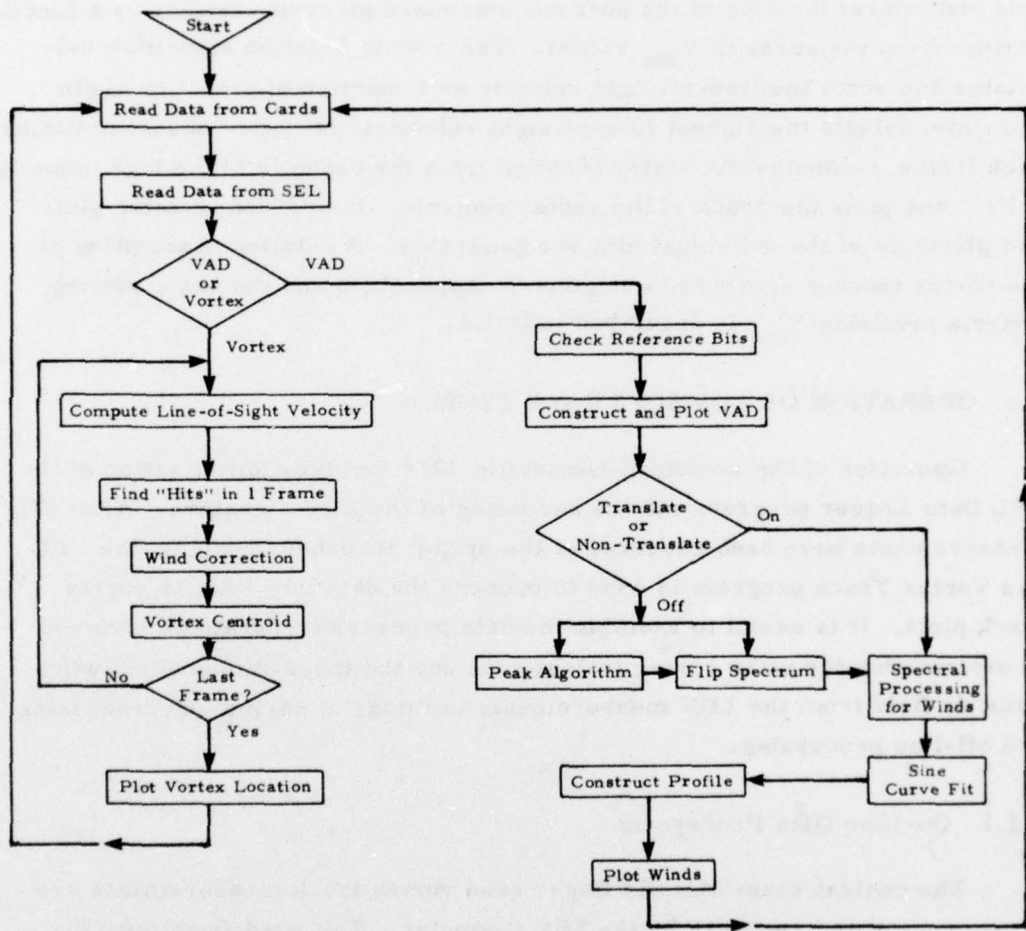
Fig. 3-5 - VAD and Vortex Track Program
