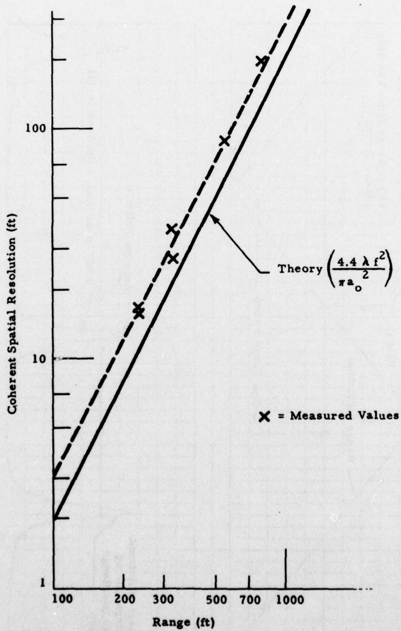
Fig. 2-18 - Field Measurements of Coherent Spatial Resolution
