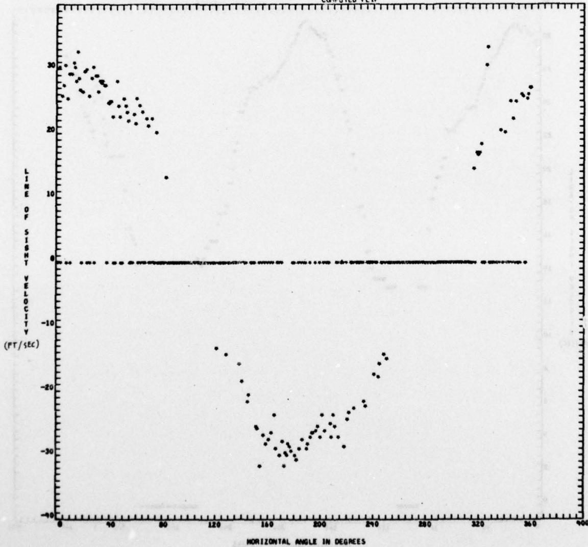
Fig. 3-10 (Concluded) c. Computed Flip of Basic Signal
