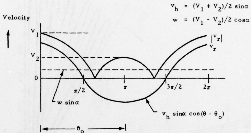
Fig. 2-14 - Azimuth Angle Dependence of Measured Velocity Component
