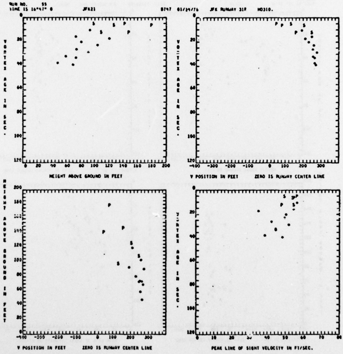
Fig.5-6 - Wake Vortex Trajectory of B-747 Aircraft - Date, 1/14/76; Time, 16:47:00
