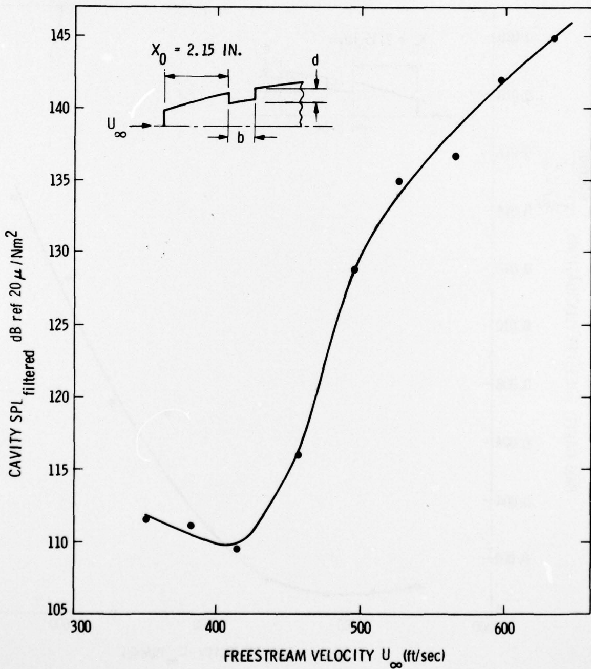
FIGURE 8. EFFECT OF FREESTREAM VELOCITY ON CAVITY SOUND PRESSURE LEVEL FOR WIDTH b = 0.3 IN. AND DEPTH d = 0.1 IN.
