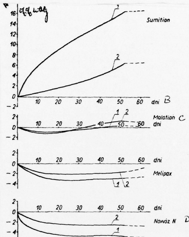
Diag. 7. Changes of polyurethane and epoxy coat weights caused by the action of SOR (plant protection agents, insecticides and fertilizers, etc.) as a function of the time of the action. 1 - epoxy set, 2 - polyurethane set, - - - changes of the coat weights during drying at room temperature.
