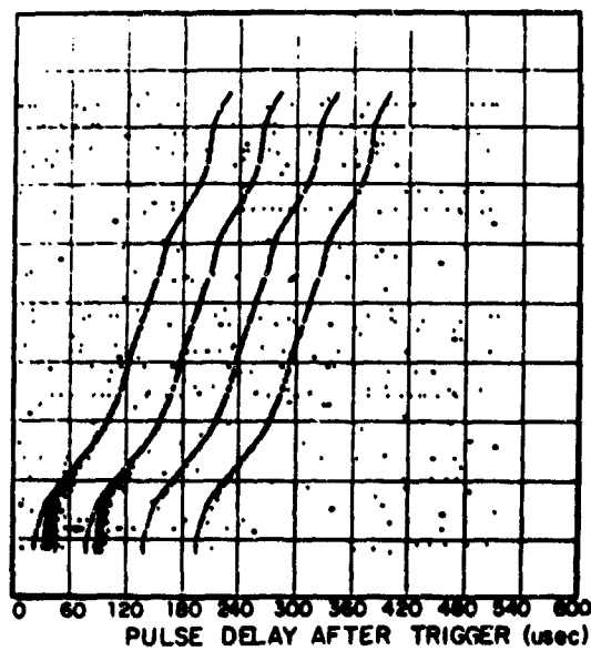
Fig. 5.24. Desert Multipath Time-Raster.
