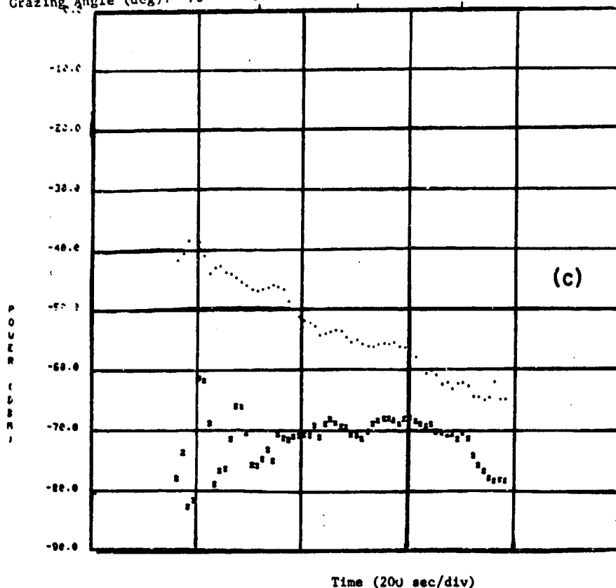
Fig. 5.7(c). Ocean (Sea State 1) Multipath Average Signal Strength.
