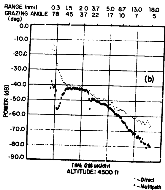
Fig. 5.7(a-b). Ocean (Sea State 1) Multipath Average Signal Strength.
