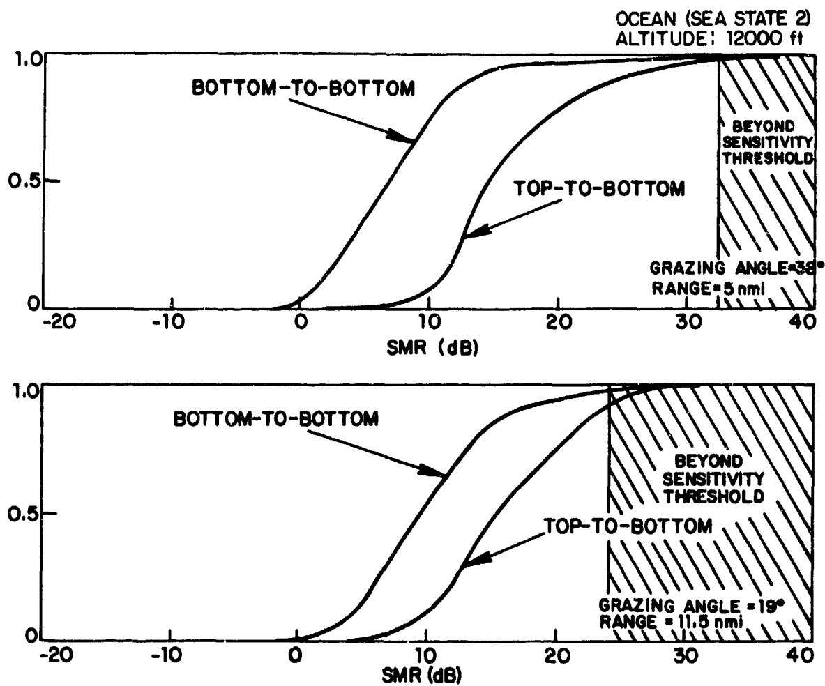
Fig. 5.12. Signal-to-Multipath Ratio Cumulative Distribution (Ocean Sea State 2).
