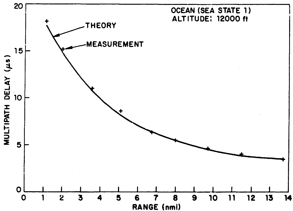
Fig. 5.3. Multipath Delay.
