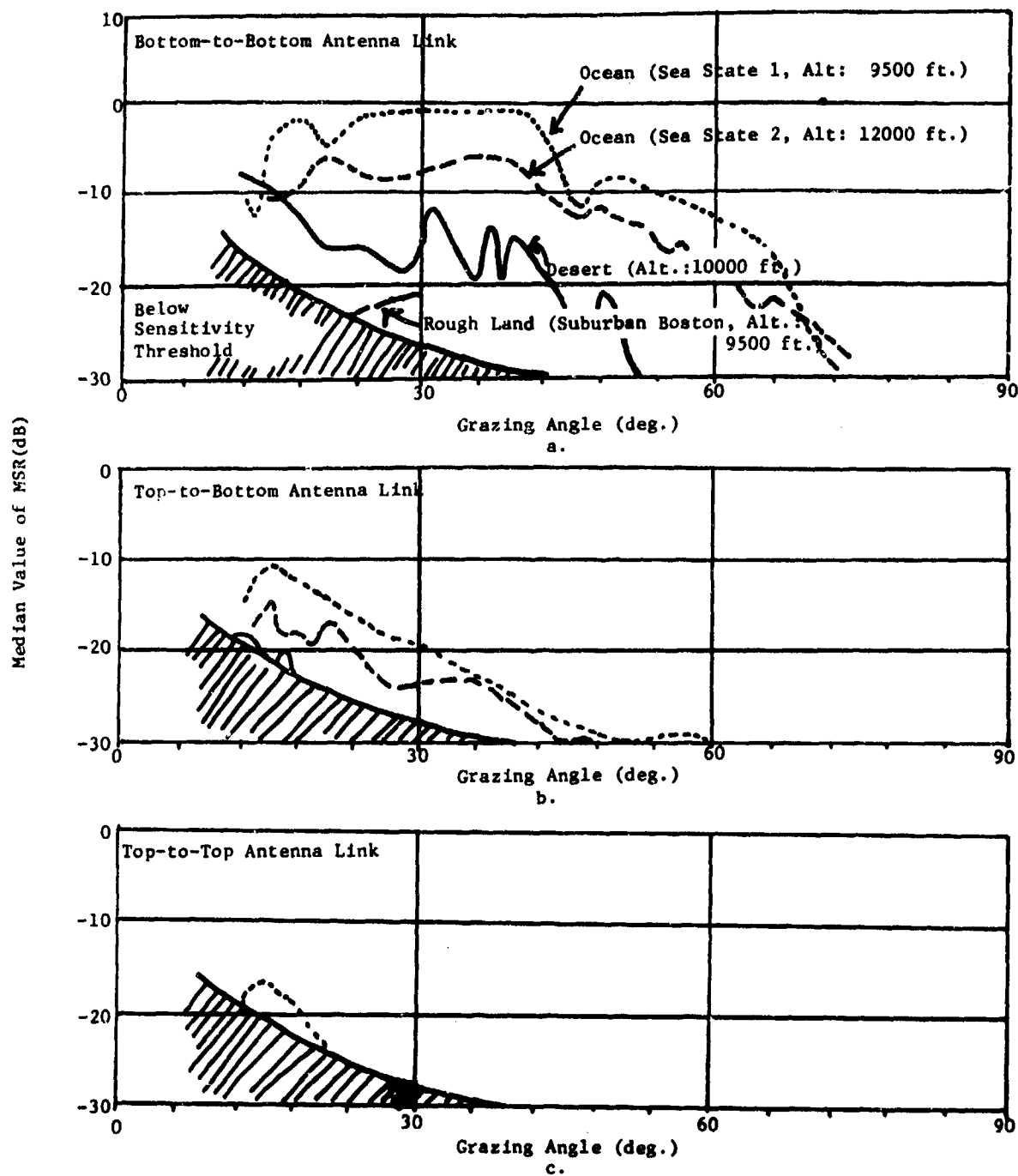
Fig. 2.1. Multipath-to-Signal Ratio Variation With Terrain.
