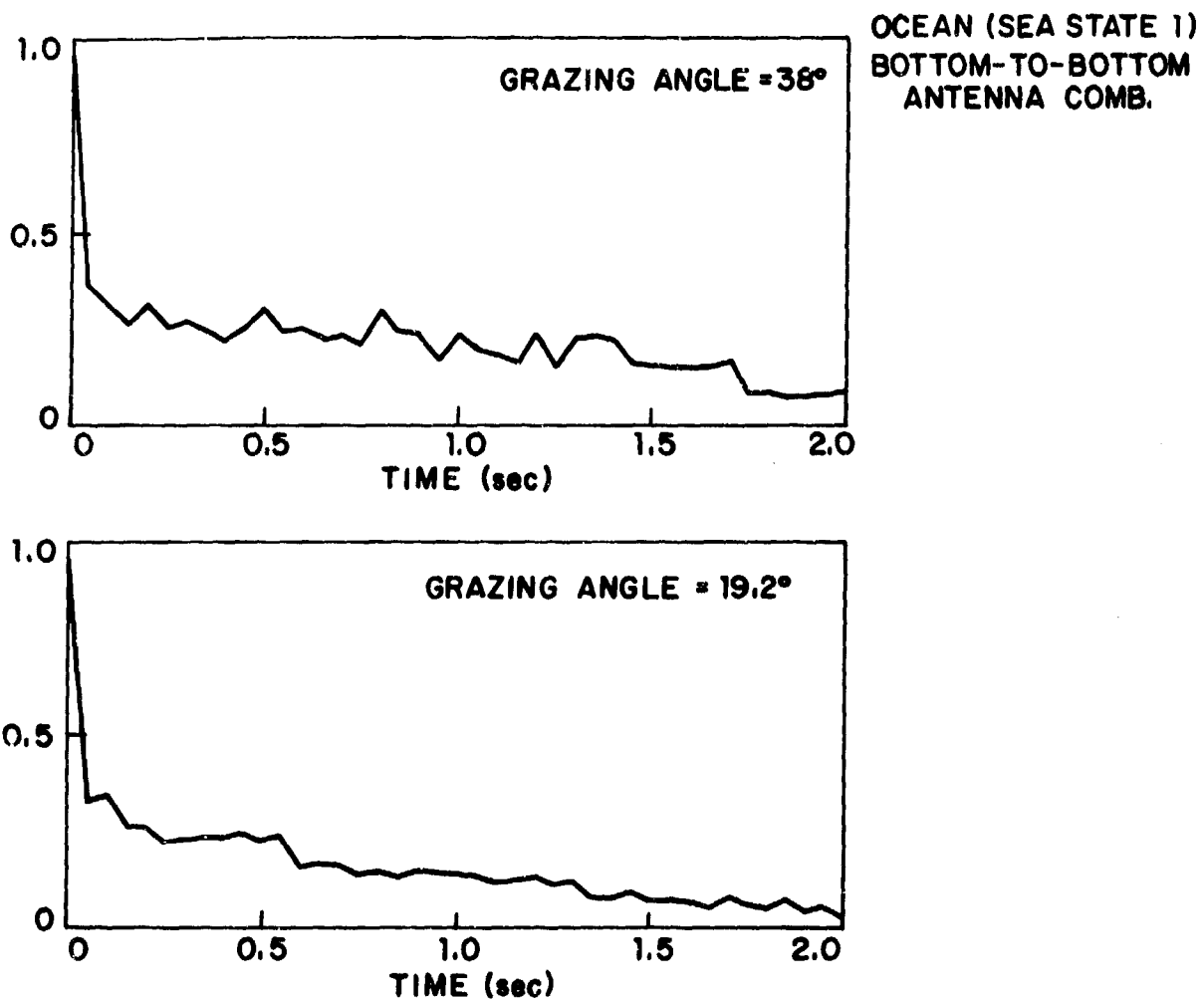
Fig. 5.5. Normalized Autocovariance (Ocean Sea State 1).
