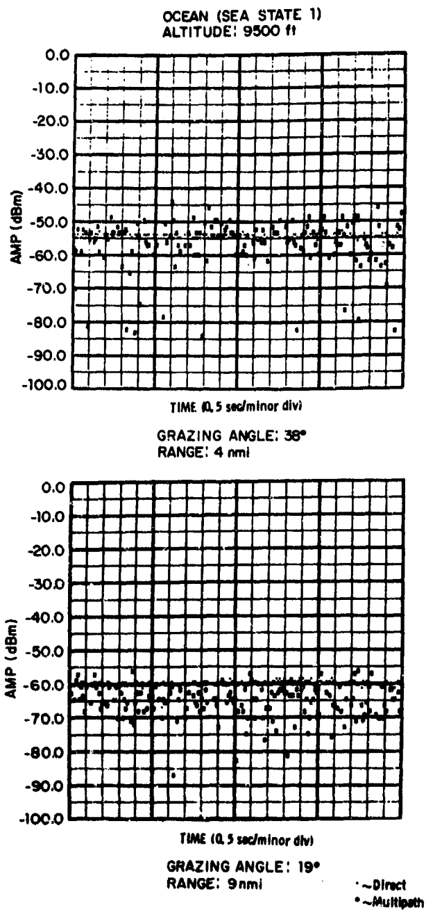
Fig. 5.4. Ocean (Sea State 1) Multipath Instantaneous Signal Strength.
