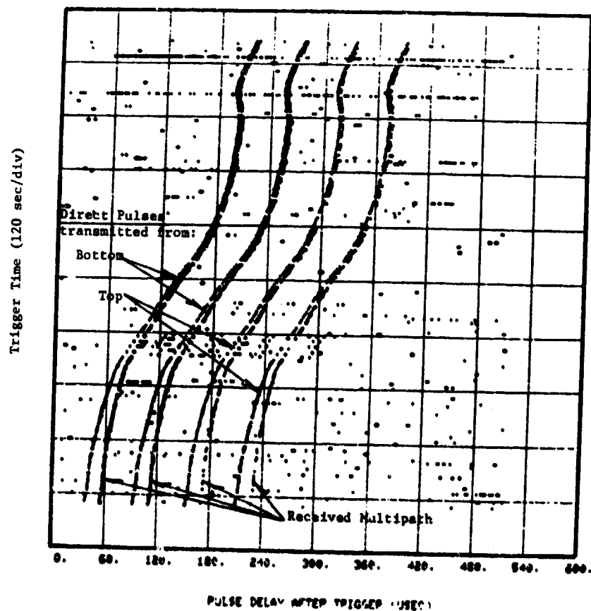
Fig. 5.2. Ocean (Sea State 1) Multipath Time-Raster.
