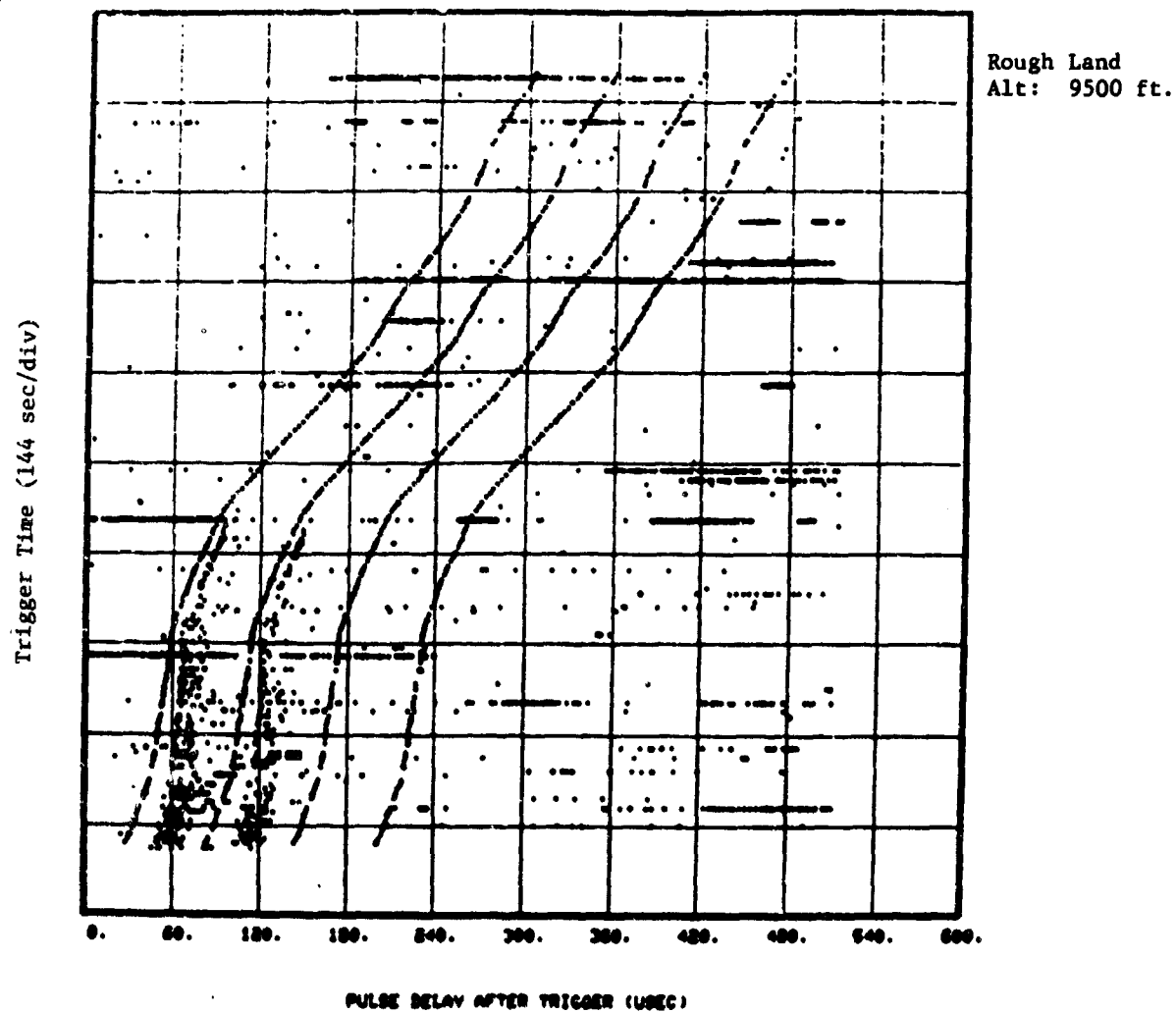
Fig. 5.34. Rough Land Multipath Time-Raster.
