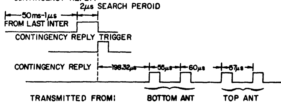
Fig. 4.5. Data Acquisition Crosslink Signals.
