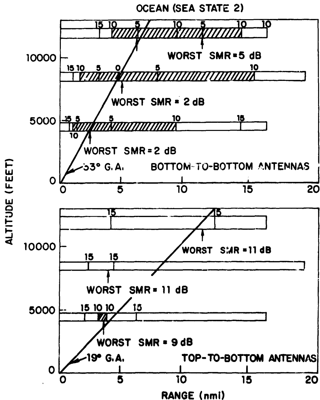
Fig. 5.17. Geometrical Dependence of Signal-to-Multipath Ratio (Ocean Sea State 2).
