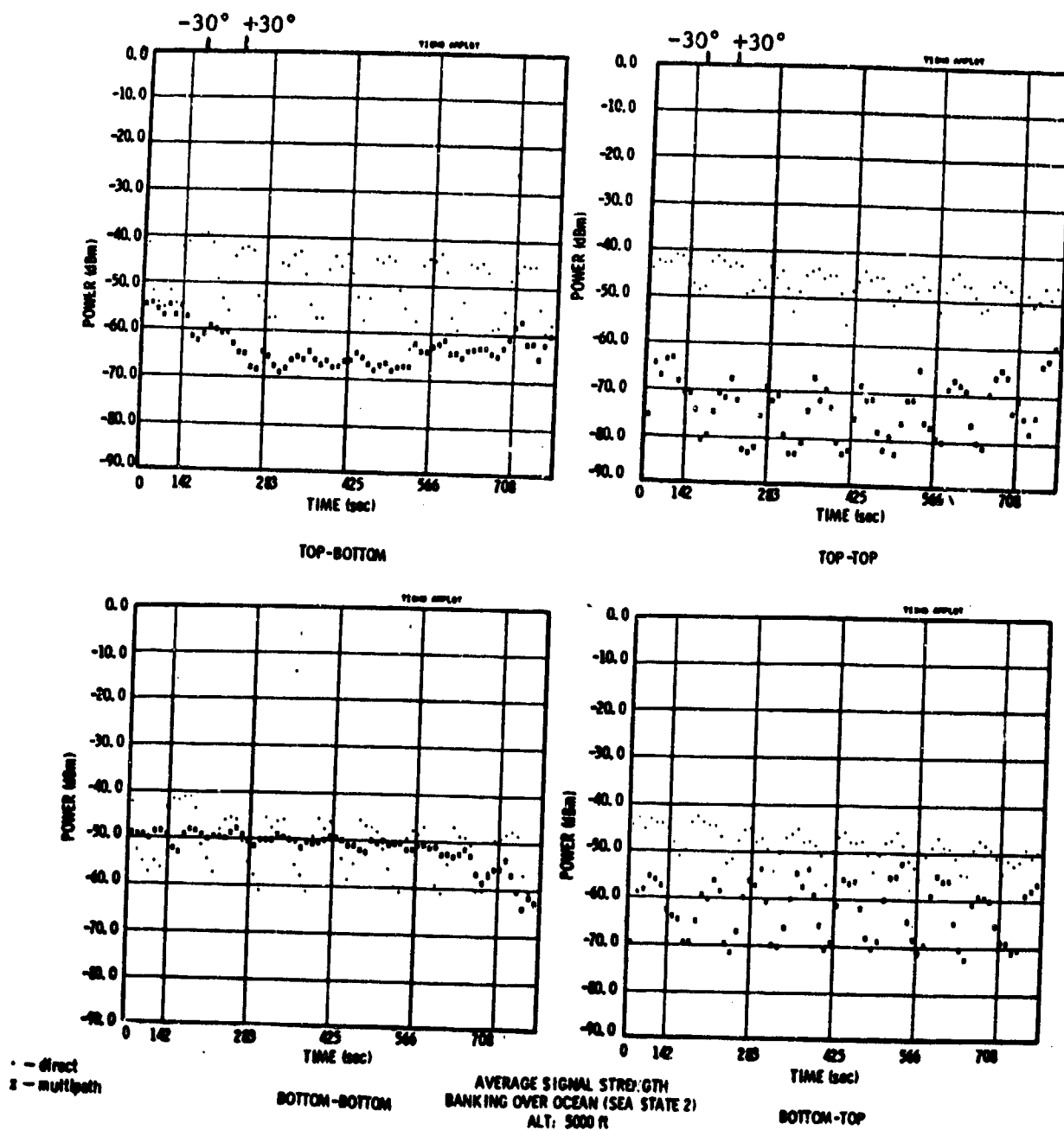
Fig. 5.39. Multipath Sensitivity to Banking.
