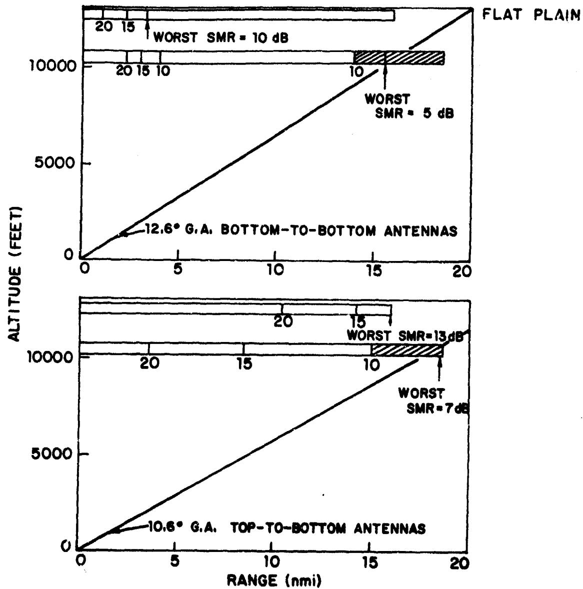
Fig. 5.33. Geometrical Dependence of Signal-to-Multipath Ratio (Flat Plain).
