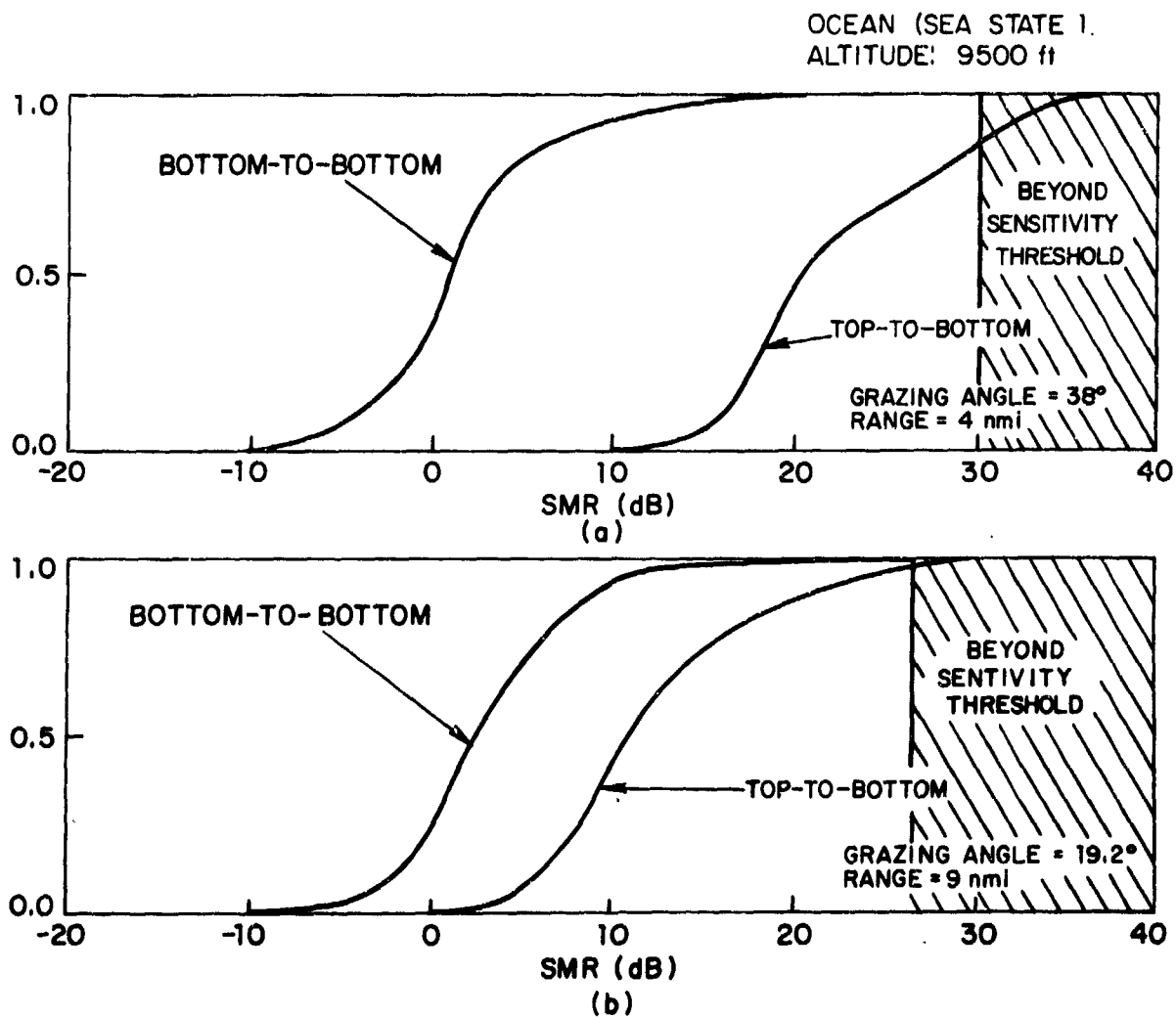
Fig. 5.6. Signal-to-Multipath Ratio Cumulative Distribution (Ocean Sea State 1).
