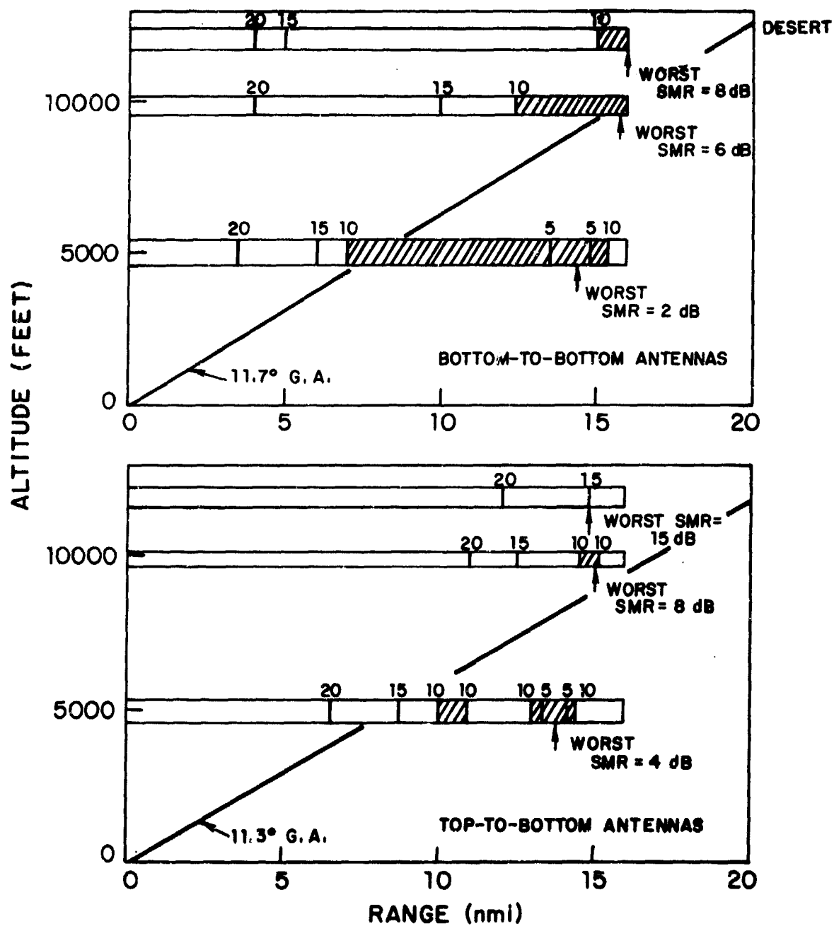
Fig. 5.32. Geometrical Dependence of Signal-to-Multipath Ratio (Desert).
