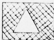
iR multiply-connected
