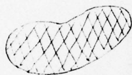
jR simply-connected
