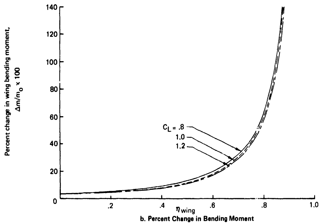
Figure 17. — Effect of AFFDL/Boeing Winglets on KC-135A Wing Bending Moment With Flaps 50^\circ
