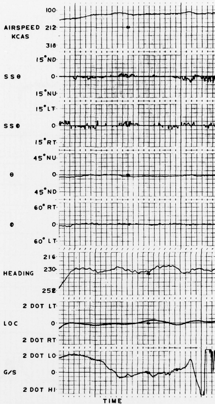
ATTITUDE COMMAND MODE APPROACH NO.3 FLIGHT 17
