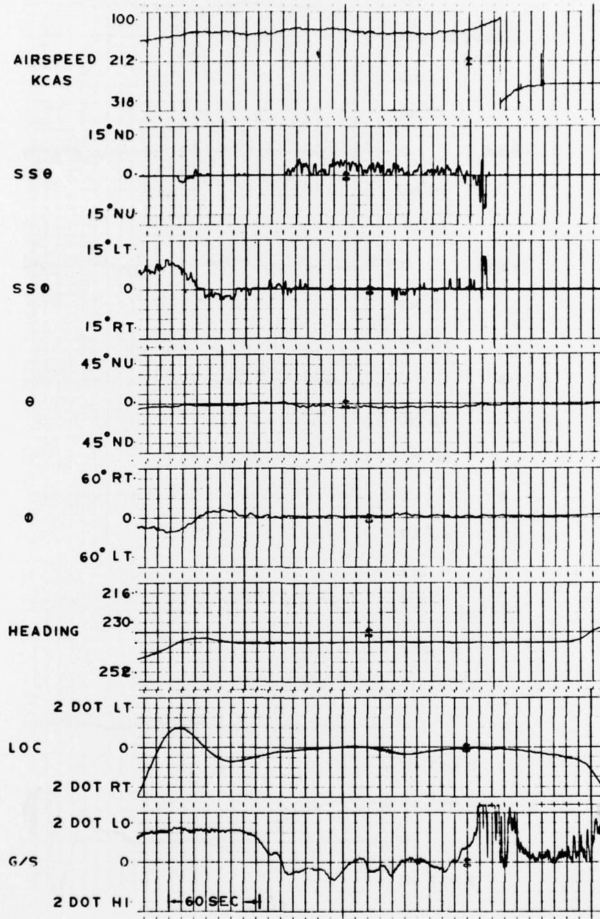
TIME ATTITUDE COMMAND MODE APPROACH AND LANDING FLIGHT 12
