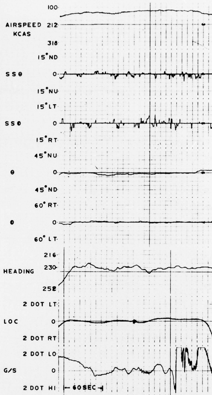
ATTITUDE CONTROL-STICK STEERING MODE APPROACH NO.2 FLIGHT 17
