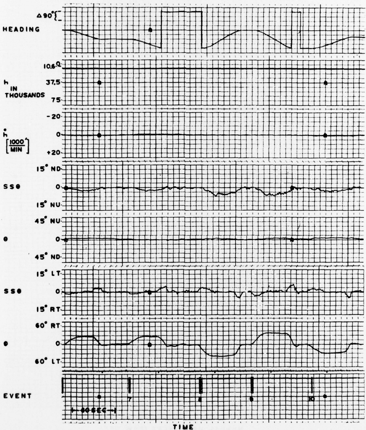
FBW MANEUVERS-ATT OFF PROJECT PILOT FLYING FLIGHT 16 FIGURE 20 42
