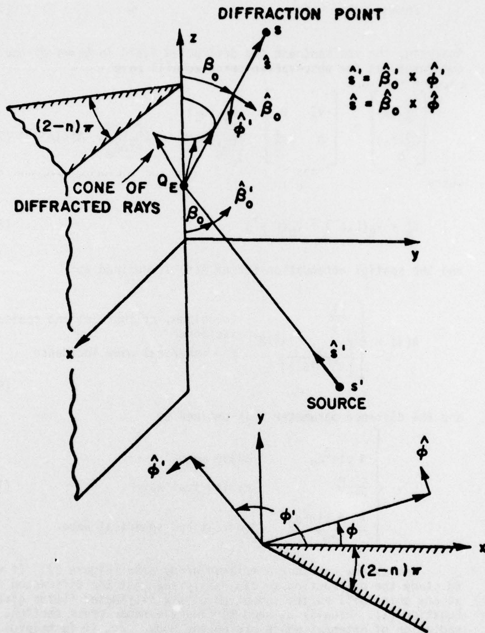
Figure 1. Geometry for three-dimensional wedge diffraction problem.
