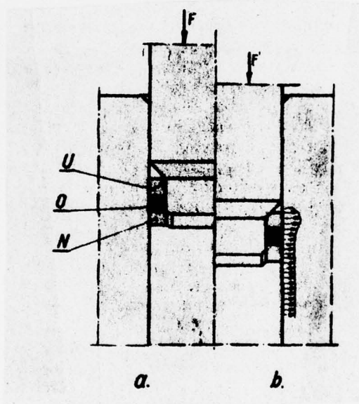
Fig. 4. Seal with uncompensated surface, supported by conicoid surface: a--initial phase of pressure exertion; b--actual seal operation under high pressure.
