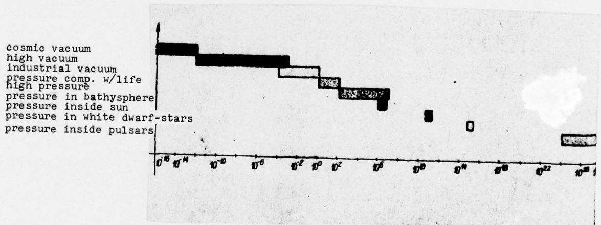
Fig. 1 Pressure Scale
