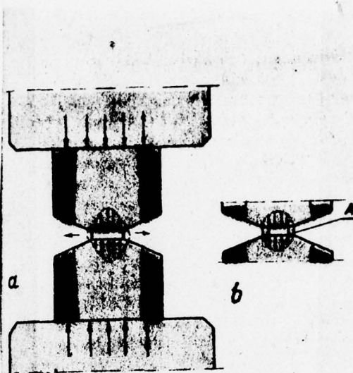
Fig. 7. Bridgman's anvil: a--cross-section of anvils together with sample piece placed between them. Arrows indicate surface pressures; b--distribution of unit of surface pressure in material placed on interior of ring and compressed by anvils.
