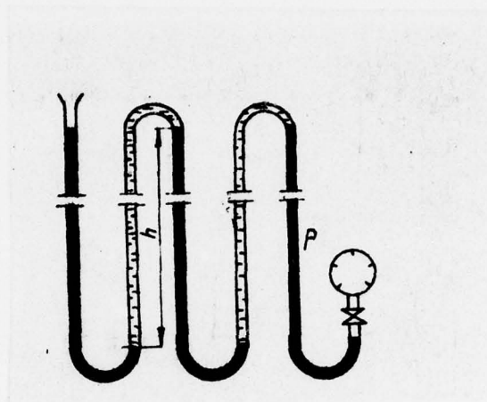
Fig. 2. Production of high pressure in a multiple mercuric column (proj. of Mendeleev). Liquid in black--mercury, with marks--oil.
