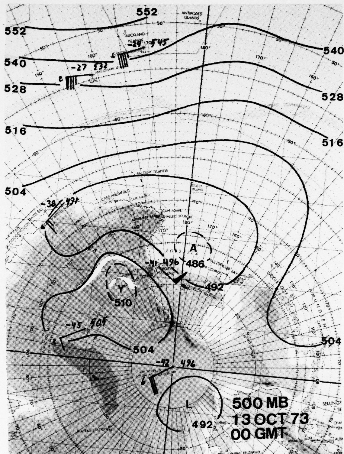
Figure 75. 500 mb analysis, 0000 GMT 13 October 1973.
