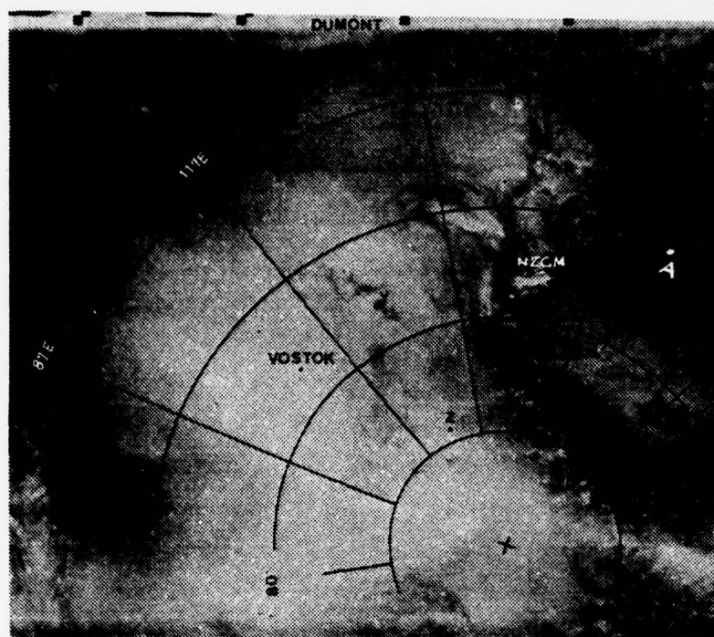
Figure 73. DMSP IR satellite observation, about 0730 GMT 12 October 1973.
