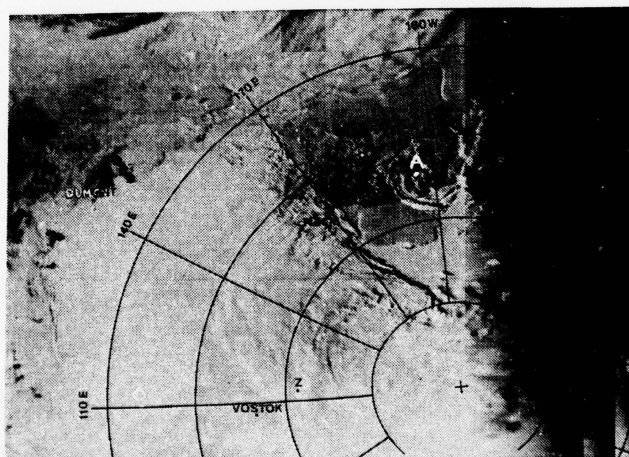
Figure 71. DMSP VIS satellite observation, about 0400 GMT 11 October 1973.
