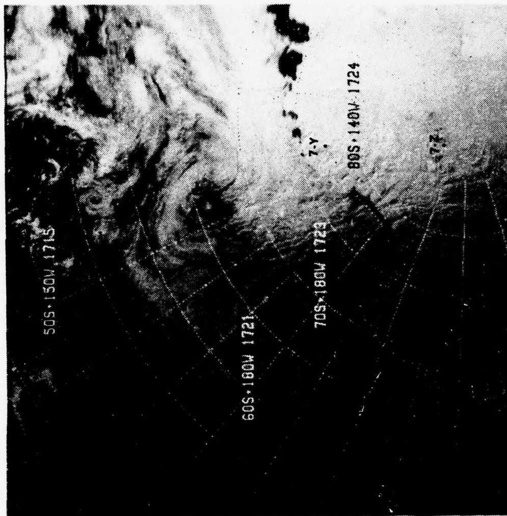
Figure 51. NOAA-4 PASS-5046 T-11 SEN-1 VIS 12/23/75 1729.
