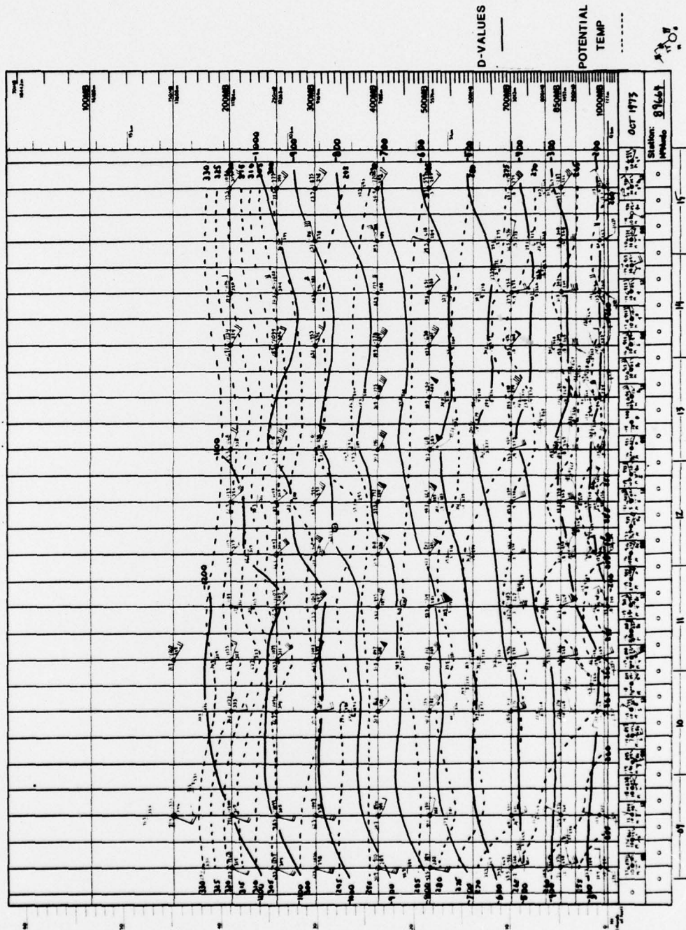
Figure 79. Vertical Time Cross-section, 9-15 October 1973.
