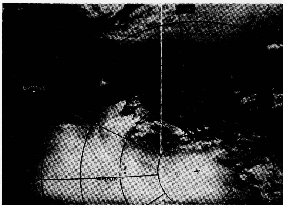
Figure 70. DMSP IR satellite observation, about 0400 GMT 11 October 1973.
