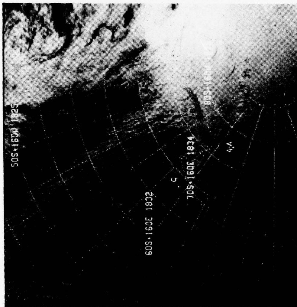
Figure 26. NOAA-4 PASS-5272 T-11 SEN-1 VLS 1/10/76 1840.
