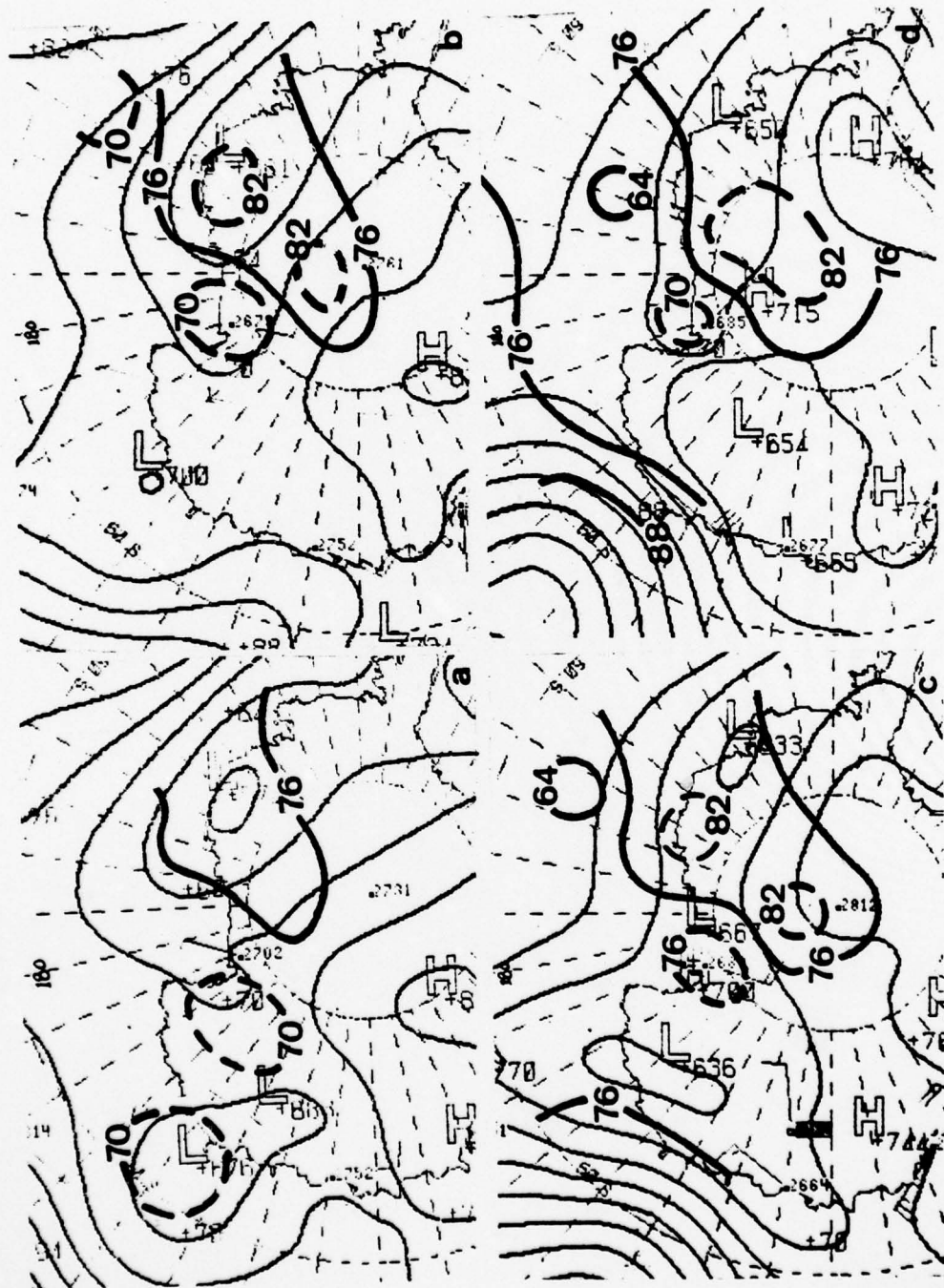
Figure 68. Comparison of FNC 700 mb analyses with those of the author. a) 22 Dec., b) 23 Dec., c) 24 Dec., d) 25 Dec. Heavy solid and dashed contours - author's analysis. Light solid, solid contours - FNC analysis.
