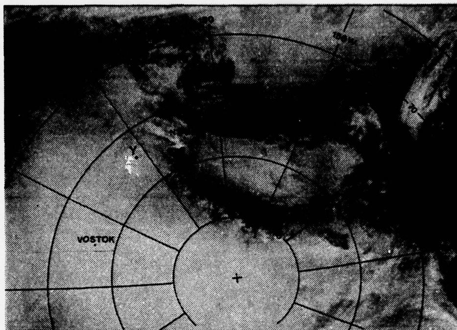
Figure 76. DMSP IR satellite observation, about 0530 GMT 13 October 1973.
