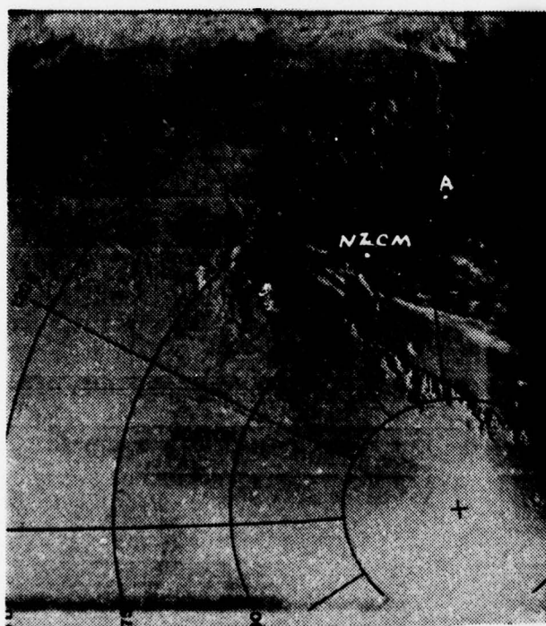
Figure 77. DMSP VIS satellite observation, about 0530 GMT 13 October 1973.
