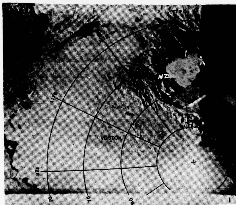
Figure 74. DMSP VIS satellite observation, about 0730 GMT 12 October 1973.
