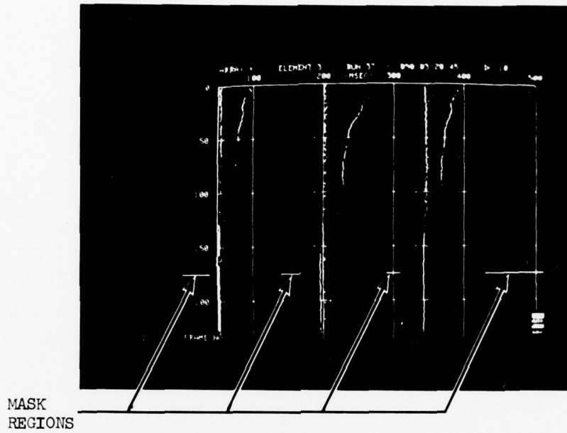
FIGURE 3-5 Acoustogram Plot (A), CRT Display
