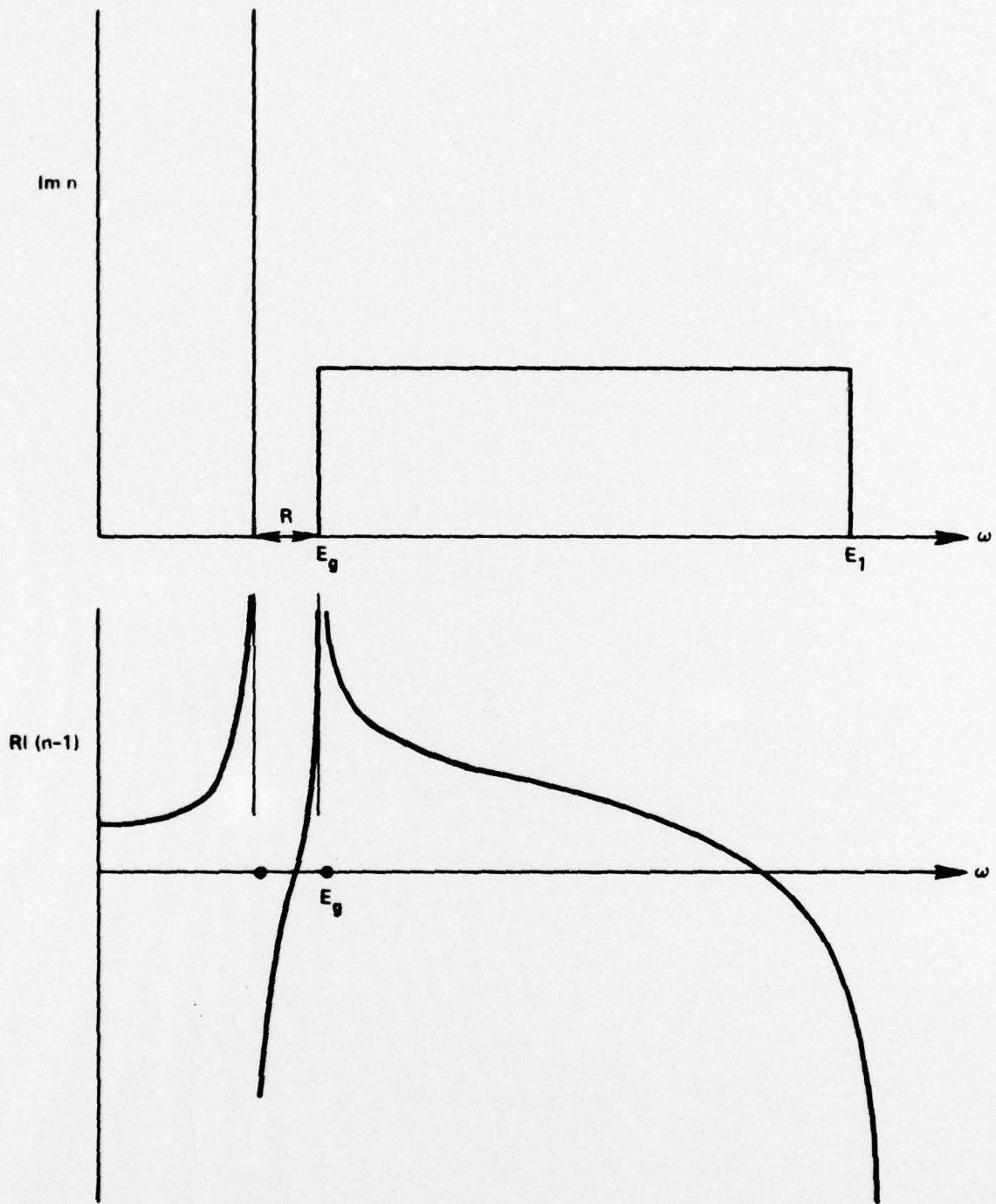
Figure 6 INDICES OF REFRACTION FOR A MODEL EDGE
