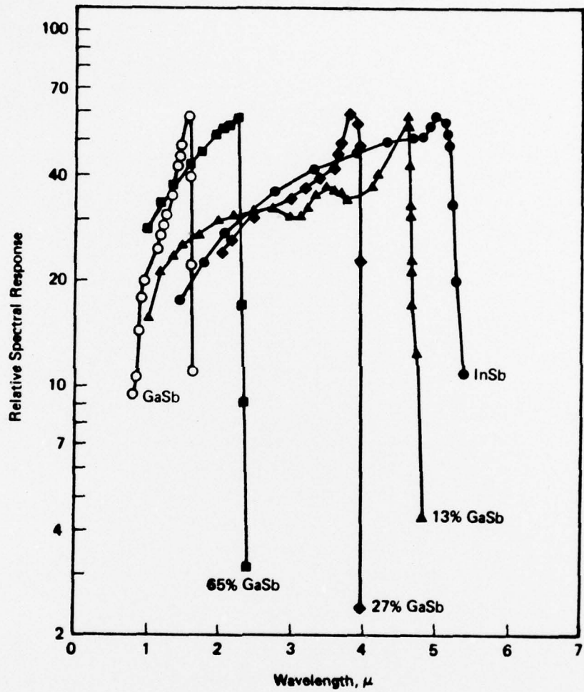
Figure 2 SPECTRAL RESPONSE OF InGaSb FOR VARIOUS FRACTIONS OF InSb. (After Wrobel and Levinstein, 1967)
