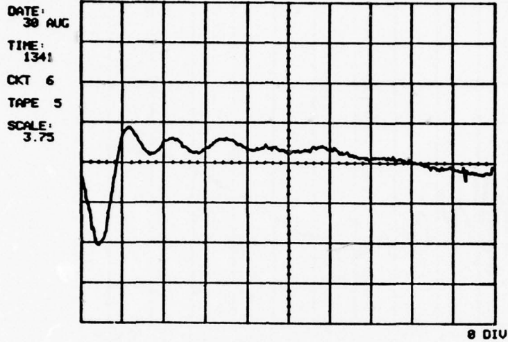
FIGURE 59. Induced Transient, Circuit 6, Power On, Slow Sweep
