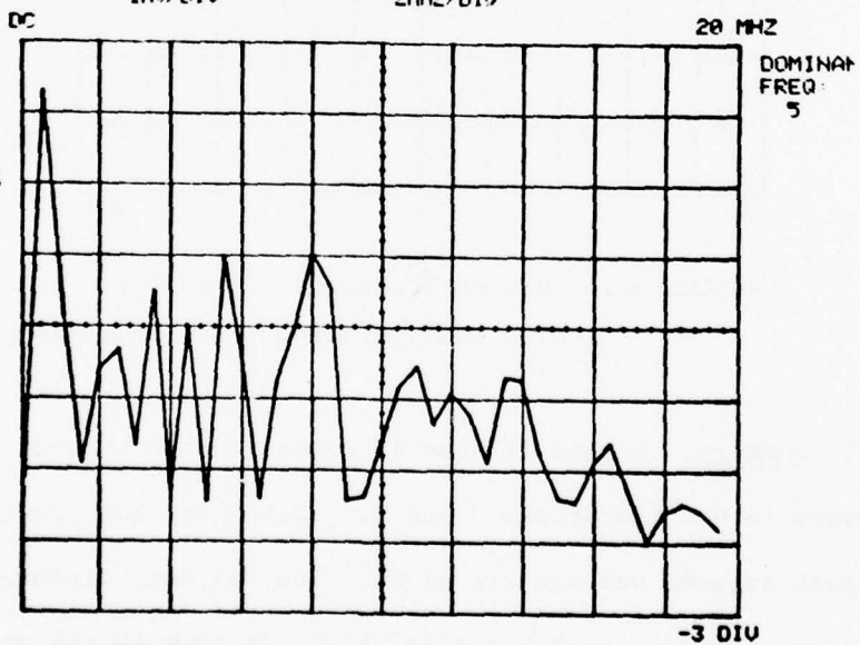
FIGURE 37. Frequency Spectrum, Circuit 6, Wire Configuration (#4)
