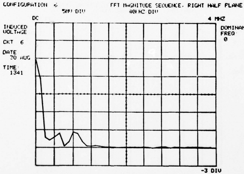
FIGURE 60. Frequency Spectrum, Circuit 6, Power On, Low Frequency
