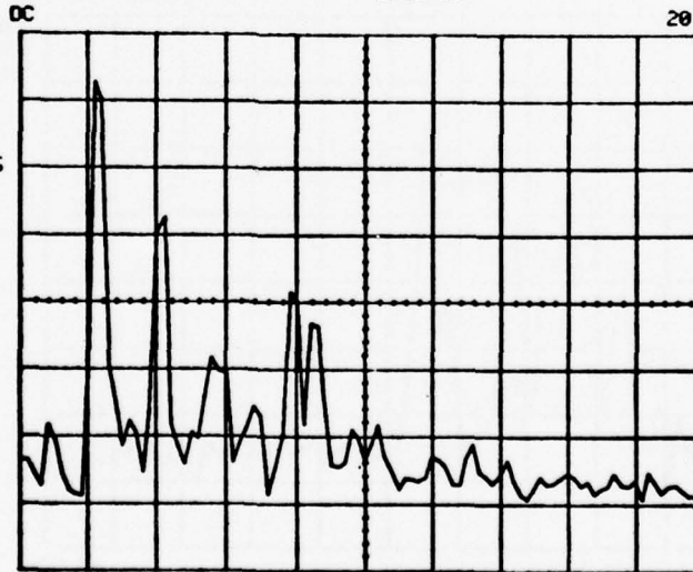
FIGURE 42. Frequency Spectrum, Circuit 1, Configuration 7
