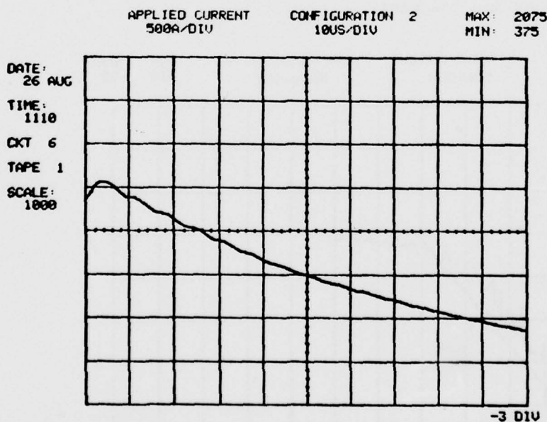
FIGURE 2. Applied Current Pulse - Overall
