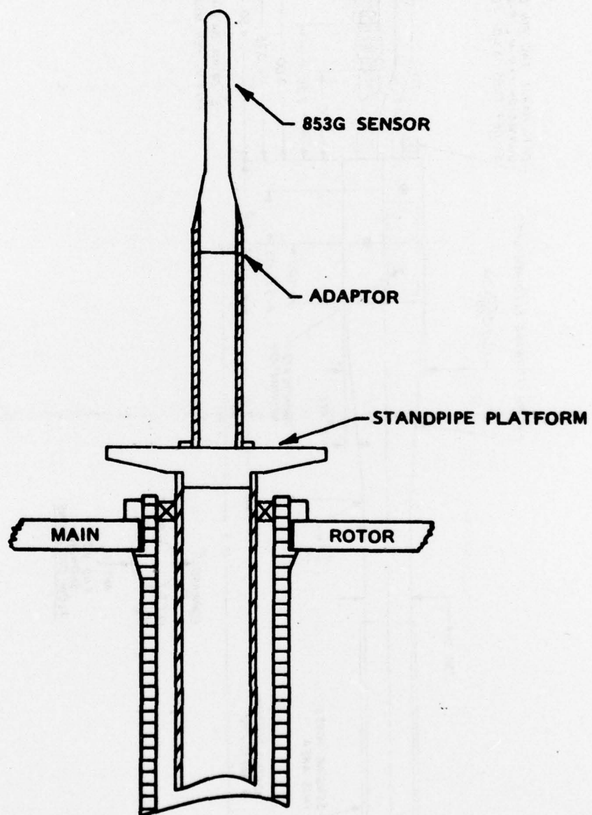
Figure 2. Sensor Installation
