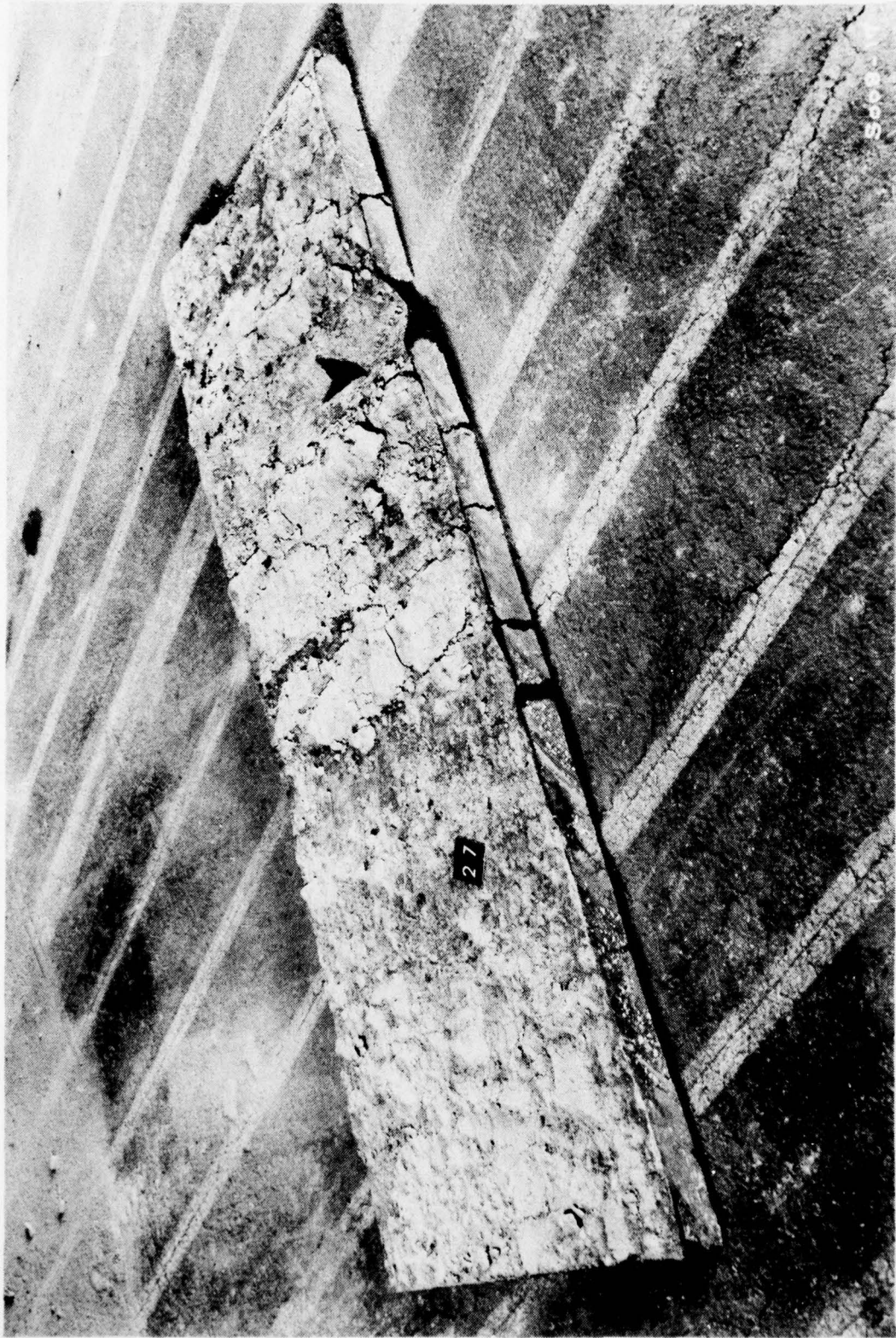
Figure 52. Wet Material That Adhered to Polypropylene Surface When Asphalt Concrete Slab Was Removed, Item 3
