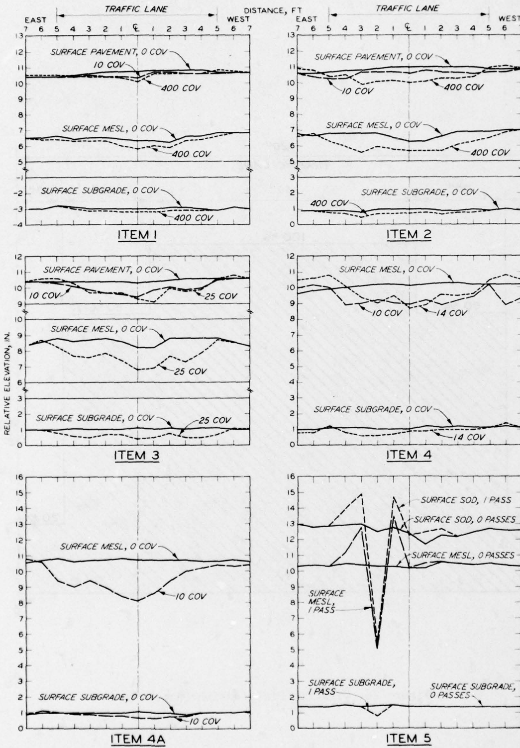
Figure 27. Typical Cross-Sections
