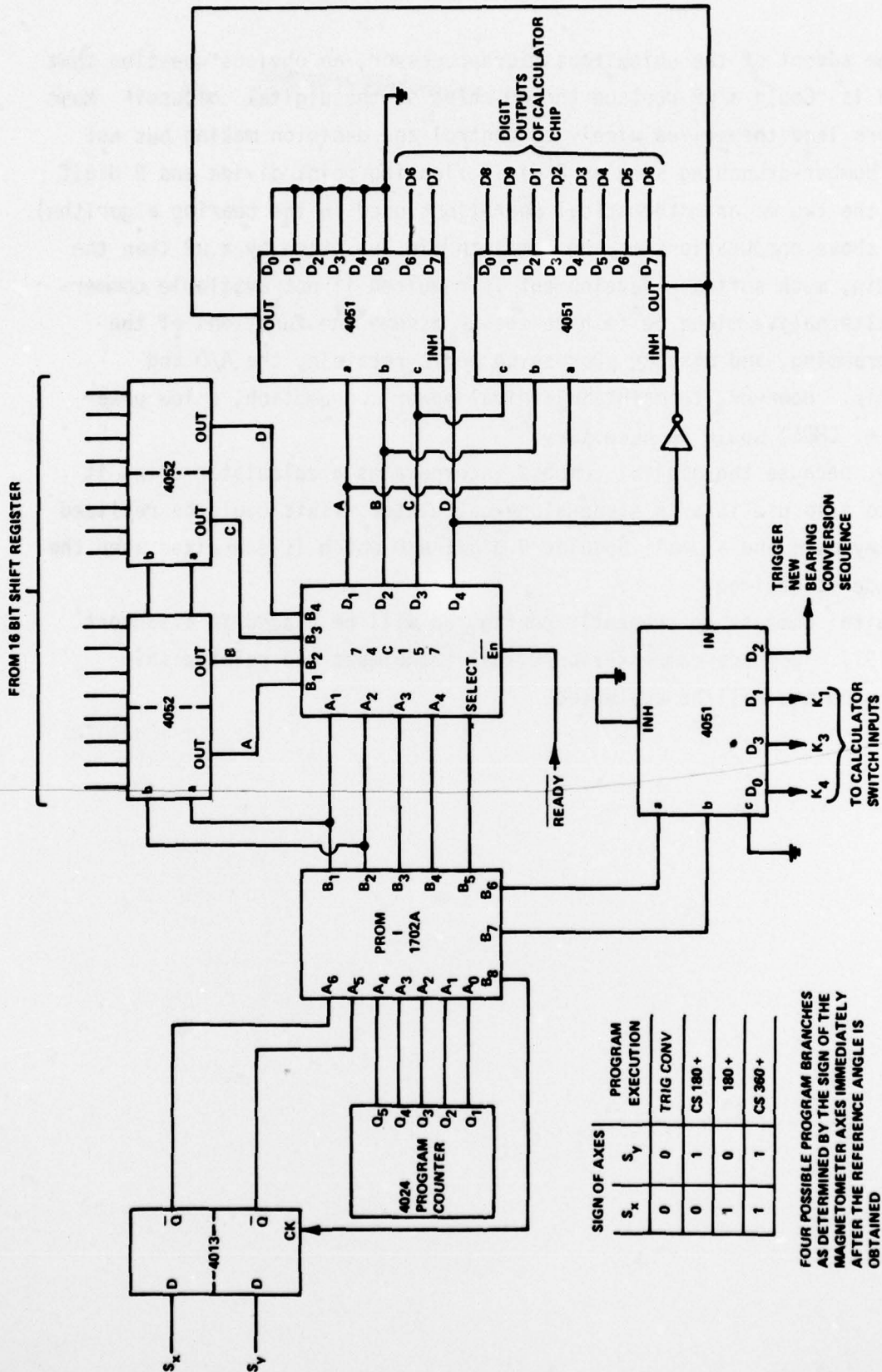
FIG. 11(U) PROGRAMMING LOGIC SIMPLIFICATION (USING ONLY 1 PROM)
