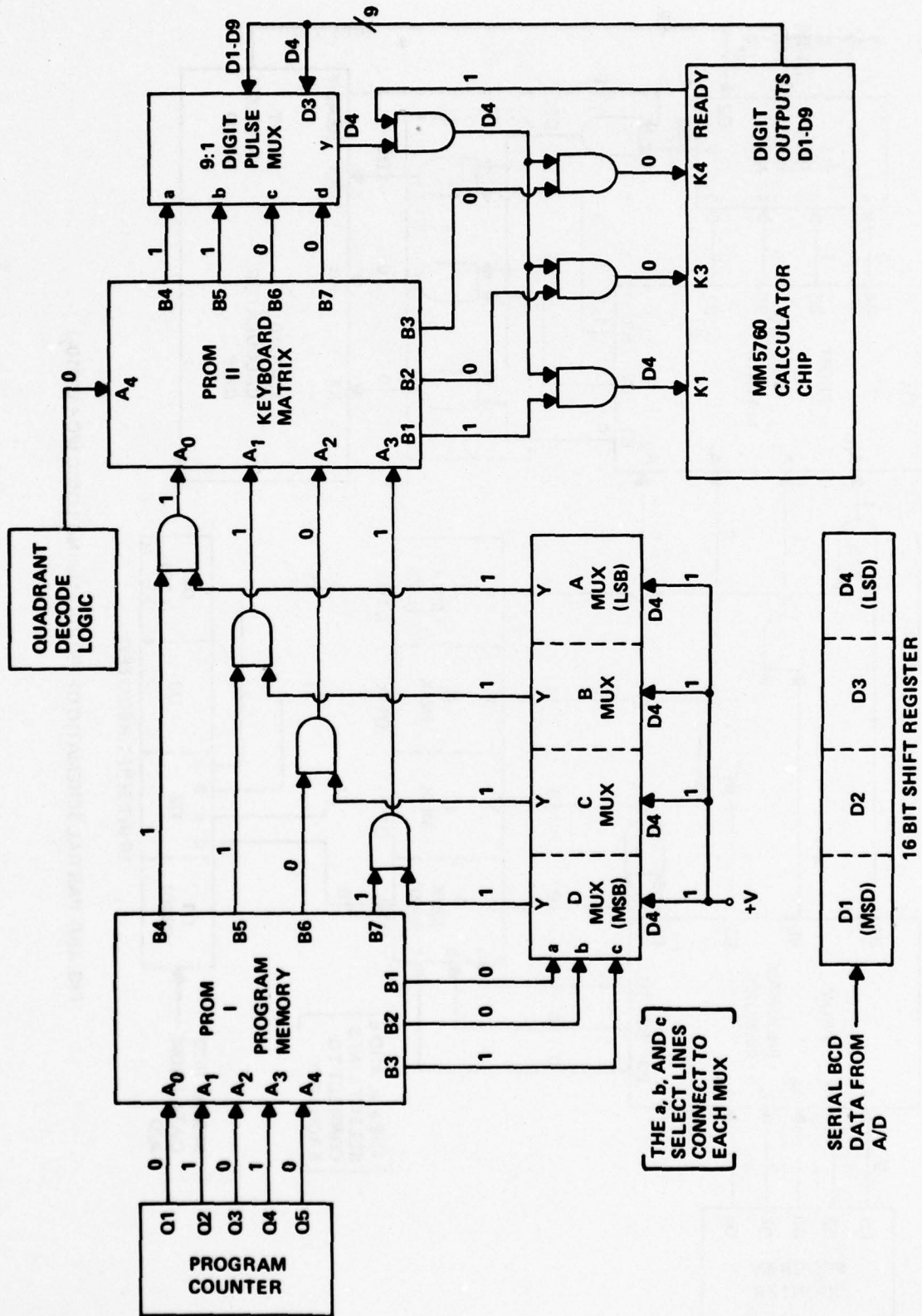
FIG. 5(U) PARTIAL SCHEMATIC OF PROGRAMMING LOGIC (PC = 01010 2 )
