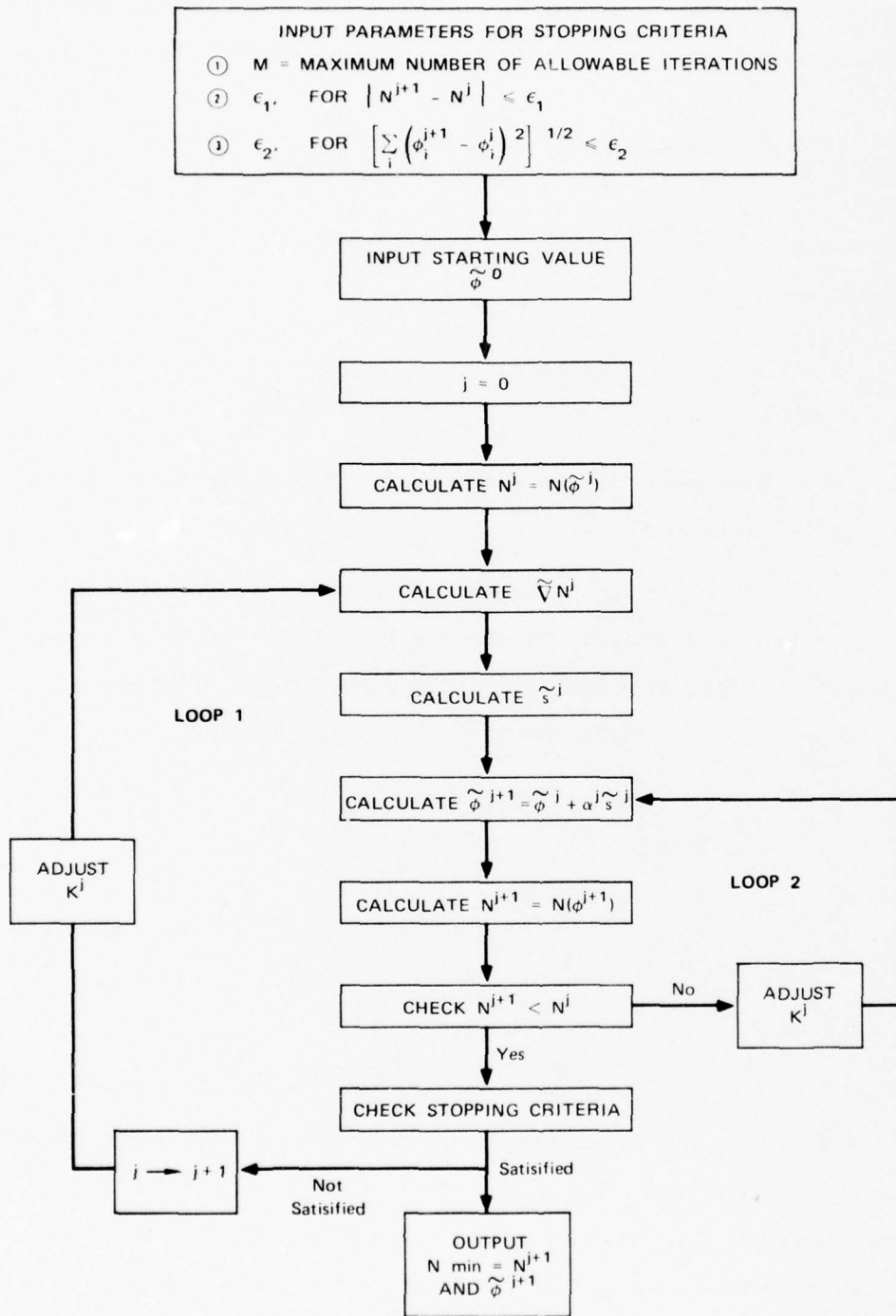
FIGURE 5 SIMPLIFIED FLOW CHART OF THE OPTIMIZATION PROGRAM STEP
