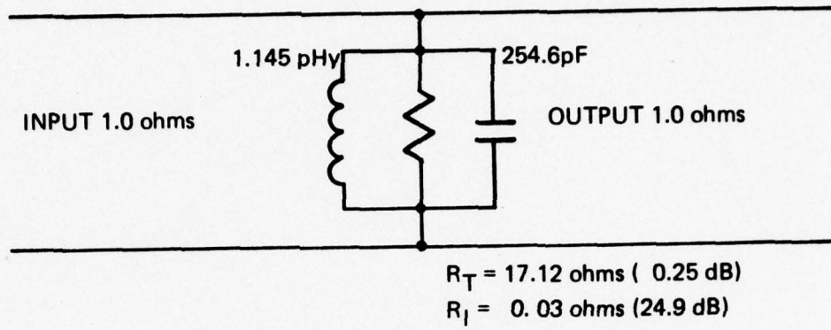
a) NORMALIZED TO 1.0 OHM
