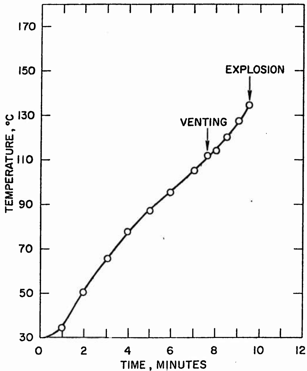
Fig. 38. Plot of the Skin Temperature of a Li/SOCl 2 D Cell as a Function of Time After Shorting the Cell Externally
