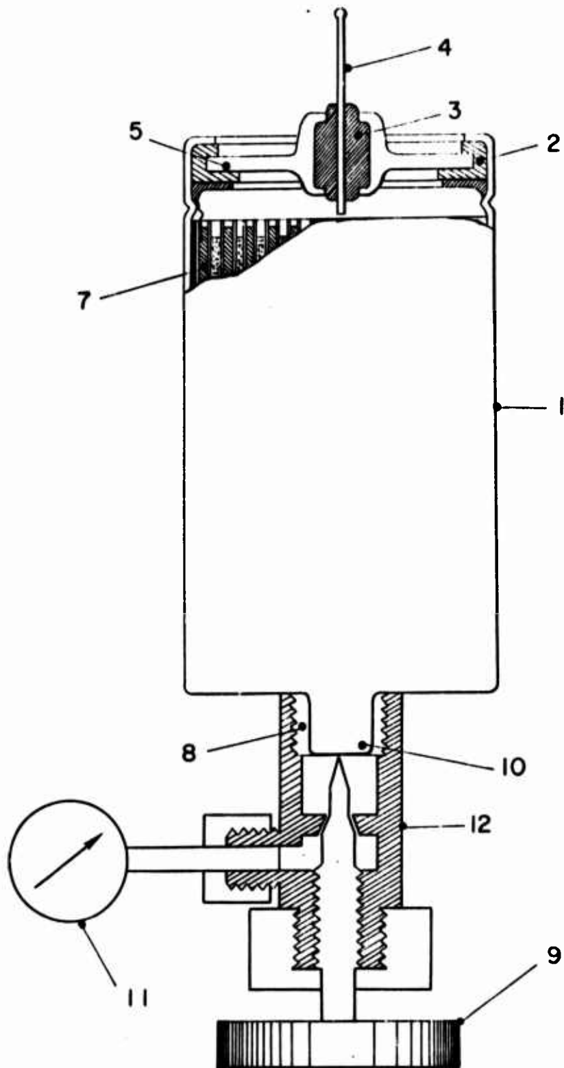
Fig. 6. Modified "C" Cell for Pressure Build-up Measurements
