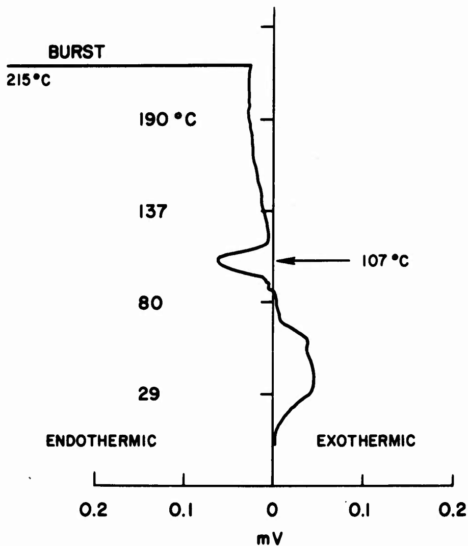
Fig. 84. Thermogram of S + 1M \text{LiAlCl}_4\text{-SOCl}_2 (90 vol%) + \text{POCl}_3 (10 vol%) Sample #90
