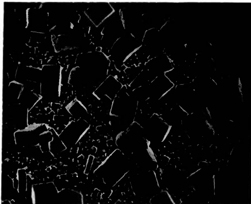
Fig. 26. SEM Photograph of Li Surface Exposed to 1.0 (M) \text{LiAlCl}_4 - \text{SOCl}_2 + 17.3% \text{SO}_2 for 8 Days at 72^\circ\text{C} . (a) 1000X (b) 200X; Film Thickness: 50 microns.
