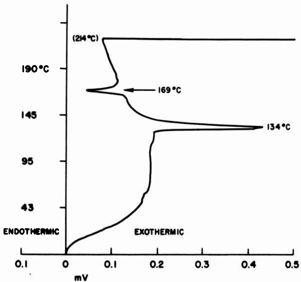
Fig. 74. Thermogram of \text{Li} + \text{Li}_2\text{S} + \text{SOCl}_2 , Sample #66
