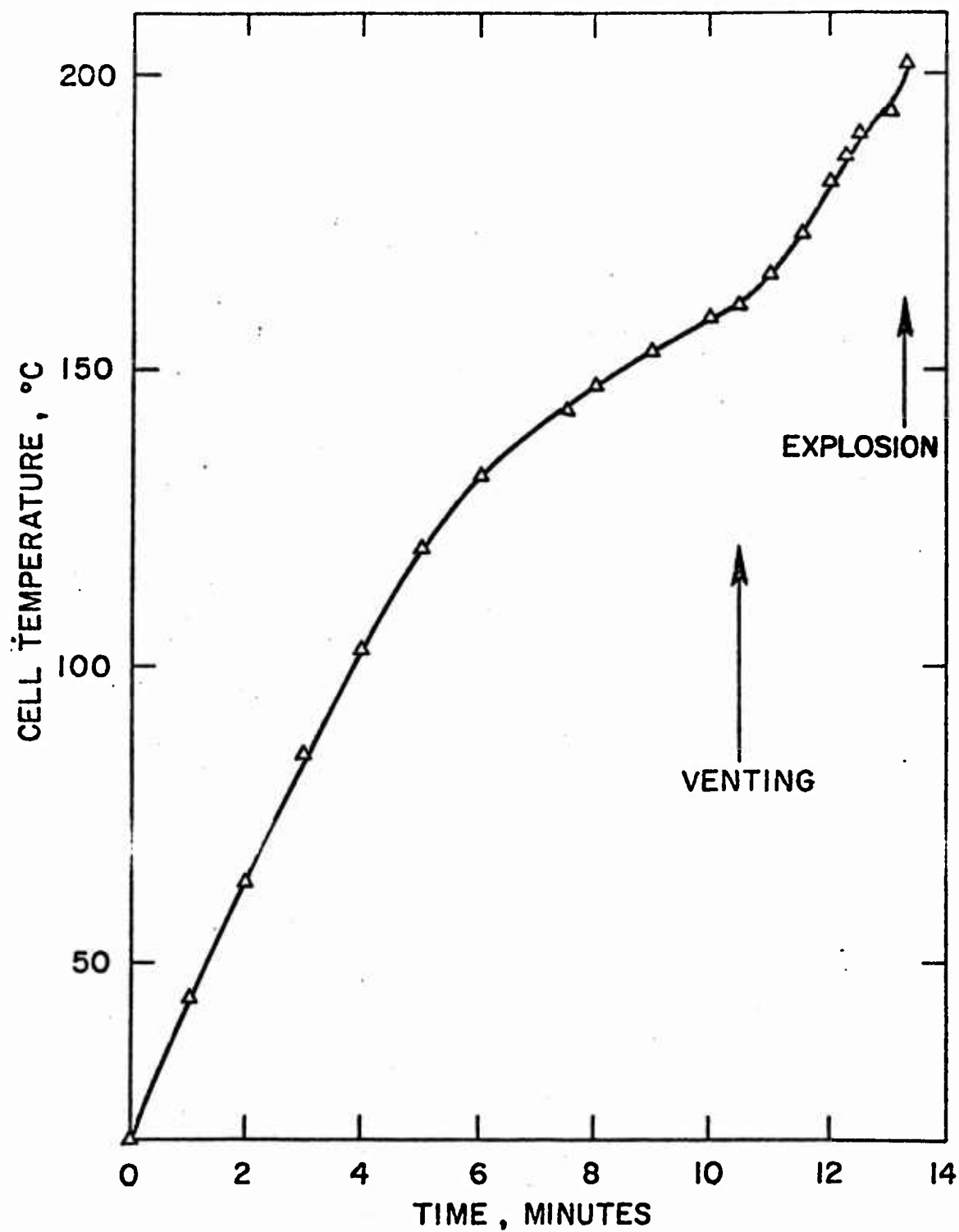
Fig. 47. Plot of the Skin Temperature of a Hermetic Li/SOCl 2 D Cell With 11.5" Electrode as a Function of Time After Shorting Externally.
