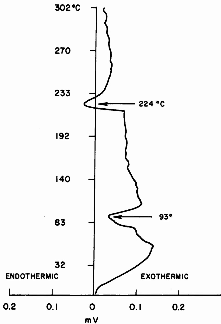
Fig. 83. Thermogram of S + 1M \text{LiAlCl}_4 - \text{SOCl}_2 (90 vol% + \text{CS}_2 (10 vol%)), Sample #89
