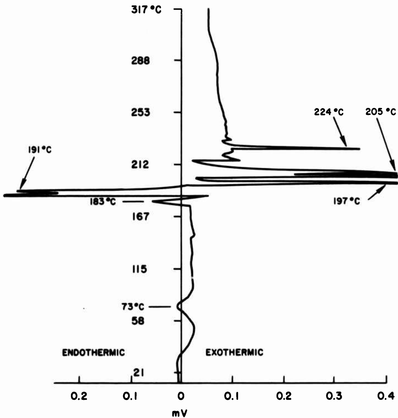
Fig. 78. Thermogram of \text{Li} + \text{S} + \text{S}_2\text{Cl}_2 , Sample #96
