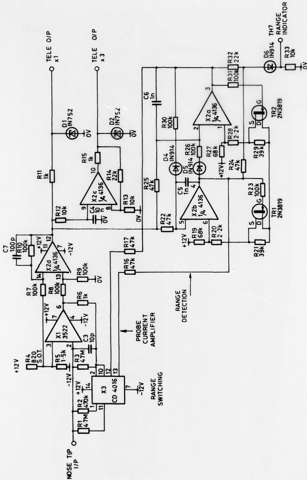
Figure 2. Circuit diagram of Langmuir probe electronics
